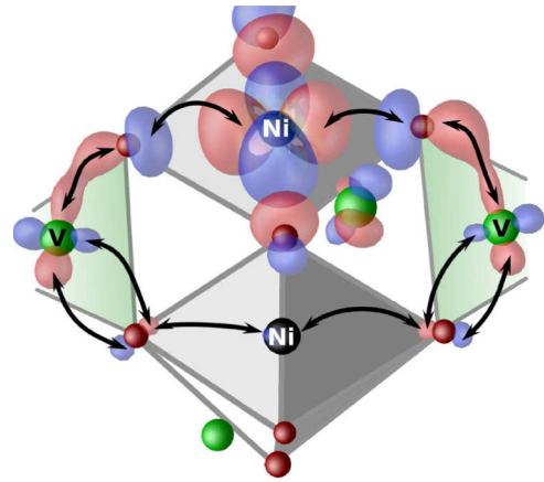
FIG. 12. (Color online) The Wannier function centered at the Ni x^2-y^2 orbital. The dominant exchange coupling J is realized by superexchange along the two inequivalent Ni-O-V-O-Ni paths indicated by arrows.
