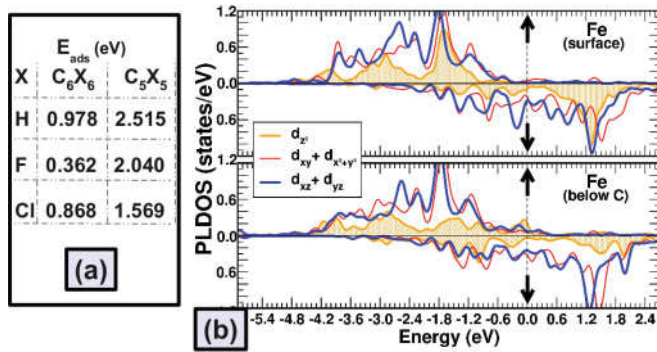
FIG. 2. (Color online) (a) The adsorption energies ( E_{\text{ads}} ) 23 show that the C_5X_5 reactive radicals interact more strongly with the Fe substrate compared to the C_6X_6 molecules ( X = \text{H, F, Cl} ). (b) The spin-resolved projected local density of states of an Fe atom of the clean surface (upper panel) and an Fe atom below the C atom of C_5H_5 (lower panel) indicate that the majority of electrons are in the spin-up channel while the minority electrons are in spin-down channel.
