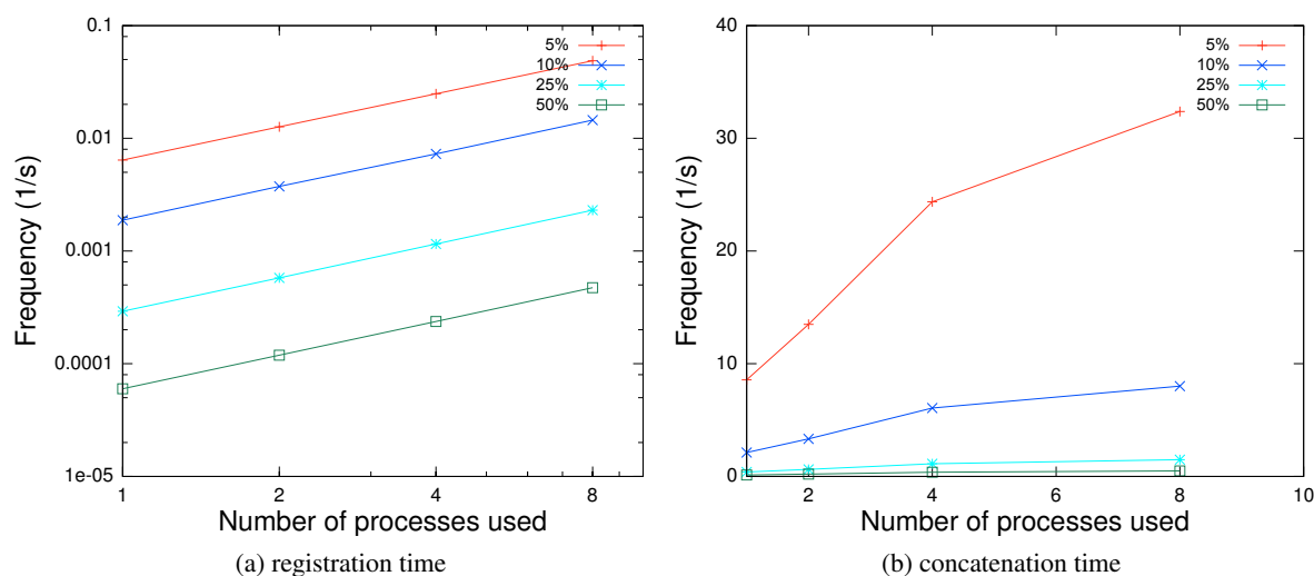
Figure 6: The left picture shows the scaling of the inverse of the registration time with the increasing number of processors. Expected scaling is O(n) . The right picture shows the scaling of the inverse of the concatenation time with the increasing number of processors.
