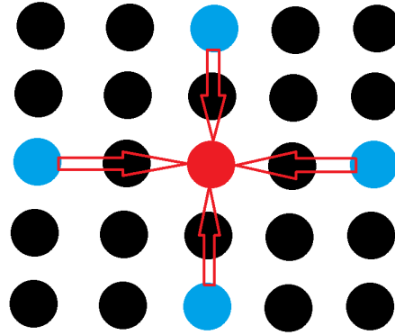
Figure 2: The new pressure for a local point is only calculated under inclusion of the next-nearest neighbours.
