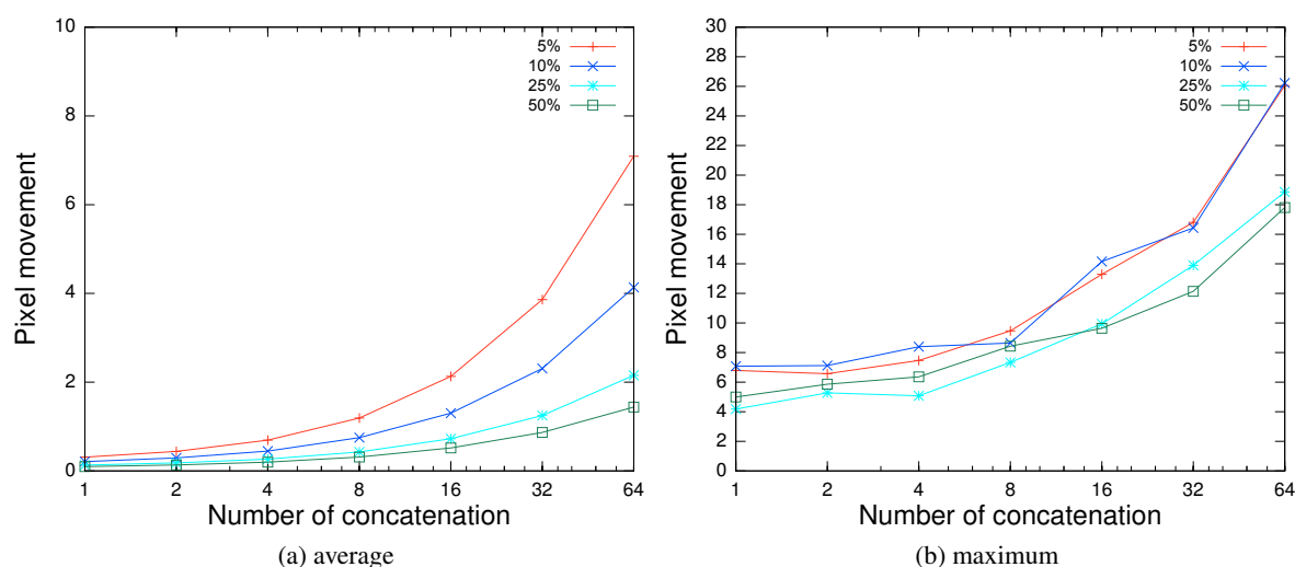
Figure 7: Average and maximum pixel movement over specified number of concatenations.
