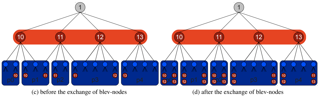
Figure 4: continued example: (c) Each process builds up the tree from the available branches of all local groups up to the level blev . (d) Globally exchange the blev-nodes and build up the tree up to the root-node. Process p0 contributes blev-node 10 and p1 contributes blev-node 11 to the global exchange. Process p2 does not contribute any blev-node, since blev-node 11 is already contributed by p1. The blev-nodes with the keys 12 and 13 are contributed by processes p3 and p4 respectively.
