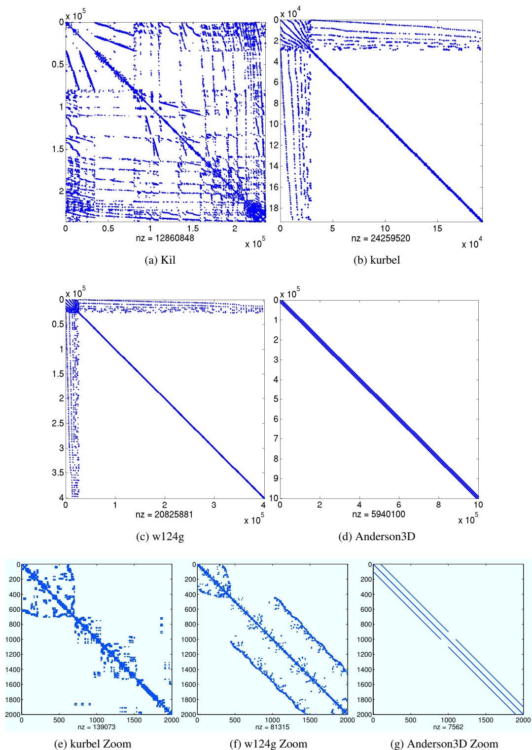
Figure 1: Sparsity patterns of test matrices
