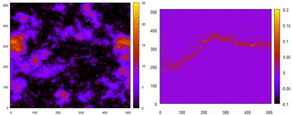
Figure 14: Left: topography with a contact area of 47.59 %. Right: Calculated current. You can see that the second path has been closed by the external force. Furthermore the current has stiffly decreased (Note the large difference in the scalebar).
