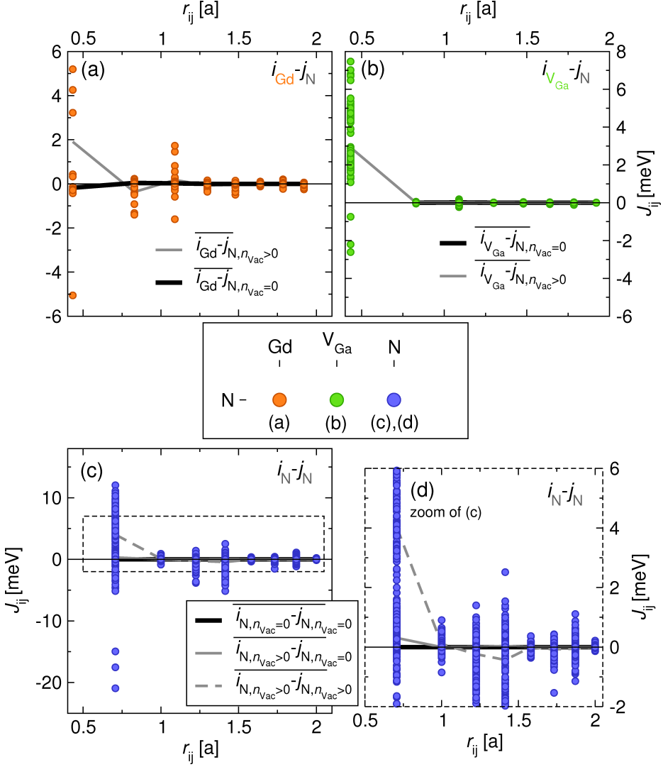
Figure 6.27.: Magnetic exchange interactions J_{ij} between (a) N and Gd, (b) N and V_{\text{Ga}} and (c), (d) N and N sites for \text{Ga}_{220}\text{N}_{256}\text{Gd}_4 . In addition to the full set of data of all interacting atoms of given kind, the mean exchange interaction to and amongst two groups of N atoms are shown (thick lines). In (a) and (b) the mean exchange constants to atoms without ( n_{\text{vac}}=0 ) and with at least one nearest-neighbor Ga vacancy ( n_{\text{vac}} > 0 ) are shown in black and gray, respectively. Accordingly, in (c) and (d) the mean interaction between N atoms with n_{\text{vac}}=0 and n_{\text{vac}}=0 , n_{\text{vac}}=0 and n_{\text{vac}} > 0 as well as n_{\text{vac}} > 0 and n_{\text{vac}} > 0 are displayed in black, gray, and gray dashed lines, respectively.
