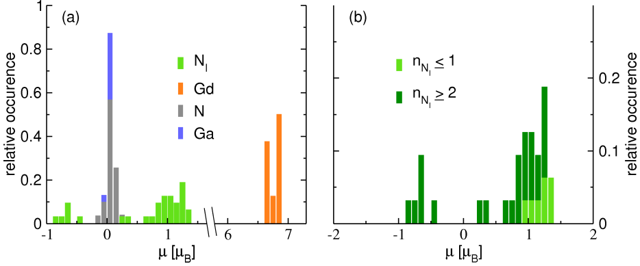
Figure 6.8.: (a) Site-specific relative probability of size and sign of the magnetic moments in Ga_{248}N_{256}Gd_8N_{1,32} . To obtain the relative probability the occurrence in all bins has been normalized by the total number of sites of the same type. In (b) the magnetic moments on N_I sites are split into two groups with respect to the occupation of its innermost three shells of interstitials. The group n_{N_I} \leq 1 experiences at most one N_I on those near interstitial sites, accordingly n_{N_I} \geq 2 at least two.
