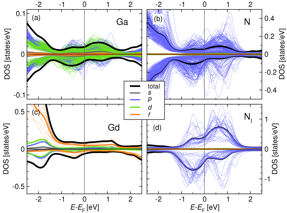
Figure 6.6.: Local density of states (DOS) of \text{Ga}_{248}\text{N}_{256}\text{Gd}_8\text{N}_{1,32} calculated with a temperature broadening of 600 K. The minority and majority spin channels are represented by negative and positive DOS values, respectively. For all Ga (a), N (b), Gd (c) and \text{N}_I sites the mean value of the orbital decomposition into s, p, d and f states is shown in relation to the mean total DOS (all in solid thick lines according to the color coding defined in the inset). In addition the individual partial DOS of p and d states for Ga (a), p states for N (b), f states for Gd (c) and p states for \text{N}_I (d) are displayed in dashed lines in the corresponding color coding.
