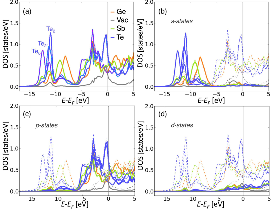
Figure 7.2.: (a) Local density of states (LDOS) of the regular ordered \text{Ge}_8\text{Vac}_8\text{Sb}_{16}\text{Te}_{32} supercell calculated with 64 k -points in Brillouin-zone and a temperature broadening of T=800 K. Te atoms are present in three neighbor configurations: zero vacancies, \text{Te}_0 (dashed-magenta), as well as two inequivalent with two vacancies, \text{Te}_2 and \text{Te}_{2'} (dashed light blue) on next-nearest neighbor sites. In (b)-(d) the partial LDOS for s , p and d states (solid lines) are shown in relation to the total LDOS (dashed lines) for the same system as in (a). In all panels Ge, vacancy, Sb, and Te-contributions are shown in orange, gray, green, and blue, respectively.
