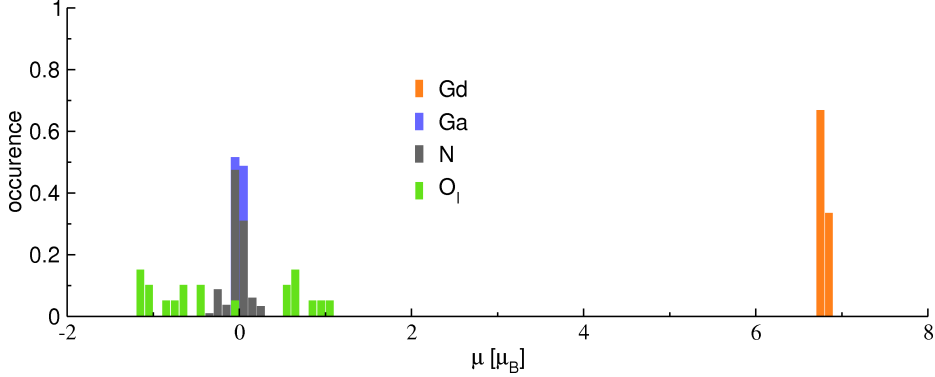
Figure 6.18.: Site-specific relative probability of size and sign of magnetic moments in Ga_{253}N_{256}Gd_3O_{I,20} . To obtain the relative probability the occurrence in all bins has been normalized by the total number of sites of the same type.
