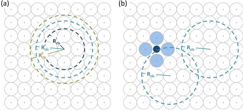
Figure 4.3.: Schematic setup of tight-binding clusters exemplary for the (001) -plane of a simple cubic lattice. In (a) different choices of cluster defining radii R^b_{cls} > R^a_{cls} > R^c_{cls} are shown resulting in 21, 13, and 9 atoms in the cluster exclusively in the shown plane. For distorted structures as visualized in (b) showing a point defect with next-nearest-neighbor relaxation different individual clusters have to be setup for each atomic center.
