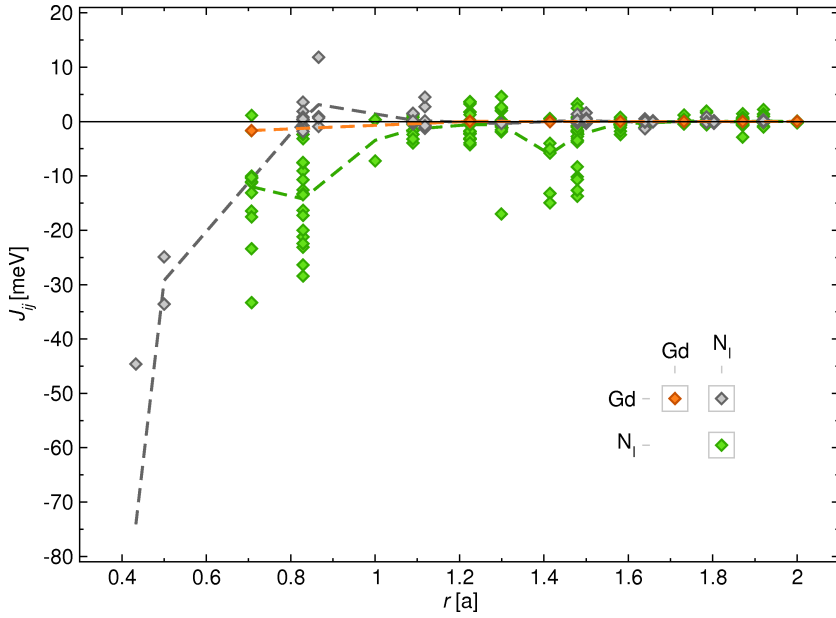
Figure 6.9.: Magnetic exchange interactions J_{ij} as obtained from the Lichtenstein-formula between Gd and Gd (orange), N I and Gd (gray) and N I and N I sites (green) for Ga_{248}N_{256}Gd_8N_{1,32} . Average exchange interactions (dashed lines) are shown for each inter-atomic distance and for all three different cases. The inset summarizes the color-coding for all three types of interactions.
