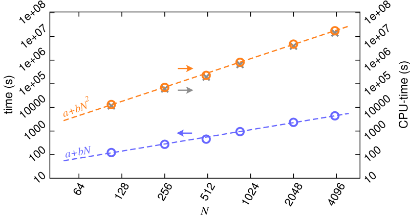
Figure 4.12.: Weak scaling, which is the scaling observed by equally increasing the system size and the number of used processors of KKRnano on JUGENE . Timings are obtained for one self-consistency step using block-circulant preconditioning of Ni_xPd_{1-x} with x \approx 3\% , one \mathbf{k} -point and l_{\max} = 3 for different system sizes. The required CPU time (orange), CPU time without communication (gray) and execution time (blue) are shown in comparison. Dashed lines are fits to the underlying data points.
