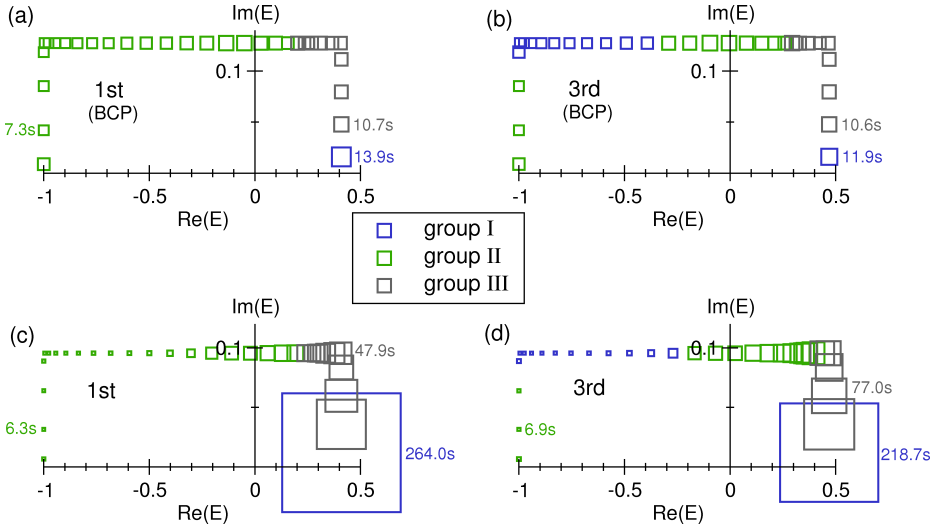
Figure 4.14.: Distribution of energy integration points as used in the energy parallelization. In (a) and (b) block-circulant preconditioning (BCP) is applied for \text{Si}_{212}\text{P}_4 with an electronic temperature of 800 K, in (c) and (d) no preconditioning is used for the same system with 600 K. The work load for each point is represented by the size of the squares. (a) and (c) show the distribution of the work load by first guess for the first self-consistency step, (b) and (d) the dynamically load balanced ones at the third self-consistency step. For selected energy points the execution time is shown.
