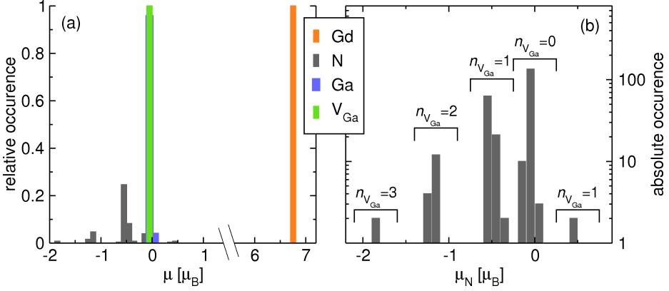
Figure 6.25.: (a) Site-specific relative probability of size and sign of magnetic moments in \text{Ga}_{220}\text{N}_{256}\text{Gd}_4 with 36 \text{V}_{\text{Ga}} in the unit cell. To obtain the relative probability the occurrence in all bins have been normalized by the total number of sites of the same type. (b) Absolute occurrence of magnetic moments on nitrogen sites, \mu_N , on a logarithmic scale. Based on the size of \mu_N N sites can be conceptually divided into four groups according to the presence of n_{V_{\text{Ga}}} = 0, 1, 2, 3 Ga vacancies on the four nearest-neighbor Ga sites.
