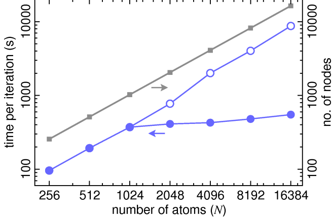
Figure 4.16.: Scaling of KKRnano in double logarithmic representation without (open blue circles) and with applied truncation (filled blue circles). The test system is \text{Ni}_{1-x}\text{Pd}_x with x = 5\% and one k -point on JUGENE. Here, parallelization over atom, spin and two groups of energy points is used. The number of processing nodes (4 CPU's per node) is shown in dark grey.
