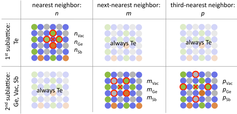
Figure 7.5.: Two-dimensional projection of the rocksalt-lattice and its disorder on neighboring sites of both the 1st-sublattice and the 2nd-sublattice occupied with Te and with Ge, Vac, Sb, respectively. The occupation with Ge, Vac and Sb on the nearest neighboring, next-nearest neighboring and third-nearest neighboring sites is described by the set of parameters n_{\text{Ge}} , n_{\text{Vac}} , n_{\text{Sb}} as well as m_{\text{Ge}} , m_{\text{Vac}} , m_{\text{Sb}} and p_{\text{Ge}} , p_{\text{Vac}} , p_{\text{Sb}} , respectively.
