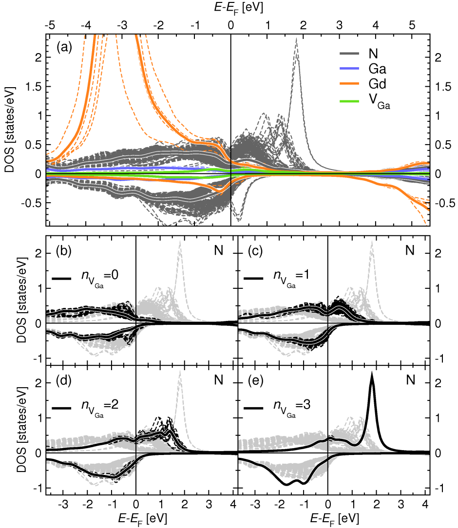
Figure 6.22.: (a) Local density of states (DOS) of Ga, N, V_{\text{Ga}} and Gd sites in \text{Ga}_{220}\text{N}_{256}\text{Gd}_4 . DOS of all sites is shown in dashed lines, the average DOS for all groups of elements in solid thick lines. (b-e) shows the DOS on N sites for different number of V_{\text{Ga}} on the nearest-neighboring Ga sites ( n_{V_{\text{Ga}}} ). Dashed black lines represent DOS on all N sites with n_{V_{\text{Ga}}} = 0, 1, 2 , and 3 in (b), (c), (d), and (e), respectively and solid black lines the average amongst those groups. Gray lines show the DOS on the remaining N sites. In all panels negative and positive DOS values represent the minority and majority spin channel.
