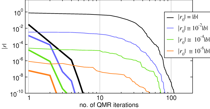
Figure 4.8.: Convergence of the residual vector |r| as a function of the number of TFQMR iterations combining the initial guess and block-circulant preconditioning for one exemplifying column of a matrix corresponding to Si_{432} . Four different qualities of starting vectors, rated by the initial residual |r_0| = Ax_0 - b are shown for comparison with (thick lines) and without applied preconditioning (thin lines). Note that a log-log scale is used.
