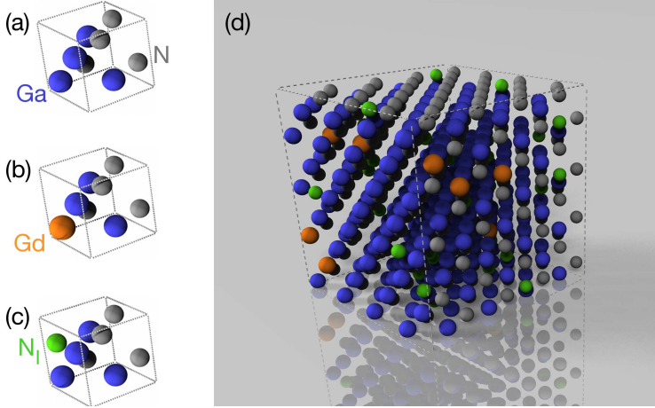
Figure 6.4.: Illustration of the fundamental building blocks of the investigated structure: GaN in zincblende structure without defects (a), with Gd on the Ga site (b) and a nitrogen interstitial ( N_I ) on a randomly selected interstitial site. In (d) the actual calculated structure Ga_{248}N_{256}Gd_8N_I_{32} is shown. For all panels Ga, N, empty interstitial, Gd and N_I are labeled in blue, gray, transparent, orange and green, respectively.
