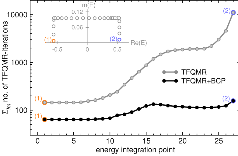
Figure 4.9.: Sum over TFQMR and TFQMR+BCP iterations for all lm components for one arbitrary atom in the test system Ni_5Pd_{251} for all 27 energy integration points. A random displacement from the ideal atomic sites on the order of 1% has been introduced. The inset shows the distribution of the energy integration points in the complex plane, the color coded points illustrate the corresponding positions of energy points in the main graph.
