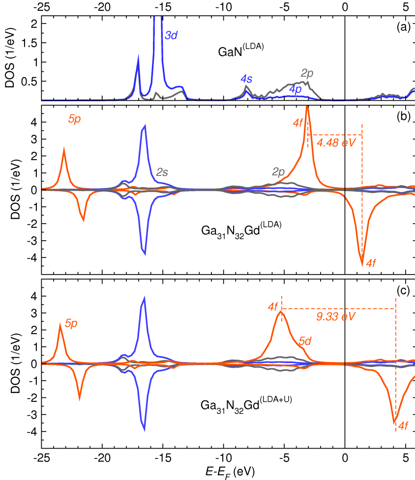
Figure 6.2.: Atom resolved density of states (DOS) for GaN (a), Ga 31 N 32 Gd 1 using the LDA exchange-correlation functional (b) and additional Coulomb-repulsion on the Gd f and d states (for details see explanation in text). The minority and majority spin channels are represented by negative and positive DOS values, respectively. For the sake of clarity the local DOS on interstitial sites is not shown and the average DOS is illustrated. In addition the position of characteristic orbitals is labeled for Ga, N and Gd in (a), (b) and (c) respectively. The characteristic splitting of the Ga 3d states is originated by the hybridization to N 2s states. Note, that the actual contour extends down to even lower energies than shown, incorporating the Gd 5s states.
