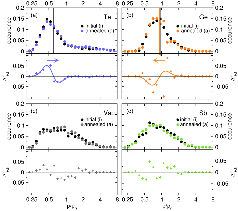
Figure 7.20.: Distribution of local density of states (LDOS) at E_F for \text{Ge}_{.25}\text{Vac}_{.25}\text{Sb}_{.5}\text{Te} supercells of 4096 sites in randomly generated configuration (i) and annealed configuration (a). All LDOS values are normalized by its mean LDOS \rho_0 . Both distributions (upper panel) and their differences (lower panel) are separately displayed for the LDOS on Te (a), Ge (b), vacancy (c) and Sb (d) sites. For all lower panels the difference as defined in the text is given in all cases relative to the initial configuration (i) supercell \Delta'_{i-a} . Lines are least-square fits according to (7.6) to the shown data points.
