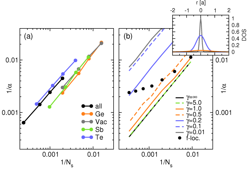
Figure 7.13.: (a) Inverse participation ratio \alpha at E_F for \text{Ge}_1\text{Sb}_2\text{Te}_4 supercells of in total 512, 1000, 1728 and 4096 sites. For the sake of comparison in (b) Gaussian distributions of states \rho(E_F) = \rho_0 \exp(r^2/\gamma) are placed randomly on 5% of the sites of a fcc-lattice with lattice constant a = 1 . Inset of (b) shows the distribution for \gamma = 0.01, 0.2 and 1.0 with the same color-coding as in (b). In the special case labeled with 'f-loc.' the number of Gaussian states ( \gamma=0.2 ) distributed on the lattice is set to 125 for all system sizes.
