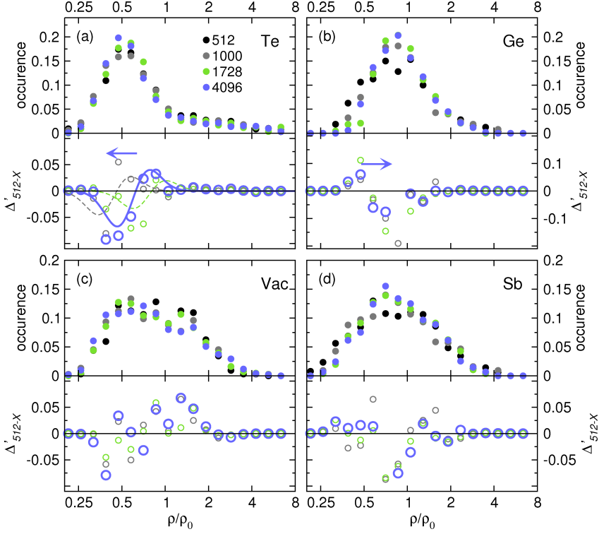
Figure 7.14.: Distribution of local density of states (LDOS) at E_F for \text{Ge}_{.25}\text{Vac}_{.25}\text{Sb}_{.5}\text{Te} supercells of in total 512, 1000, 1728 and 4096 sites in 5, 4, 3, and 1 different randomly generated configurations. All LDOS values are normalized by its mean LDOS \rho_0 . Both the distributions (upper panel) as well as its differences (lower panel) are separately displayed for the LDOS on Te (a), Ge (b), vacancy (c) and Sb (d) sites. In all upper panels of the subplots the color coding is used as specified in (a). For all lower panels the difference as defined in the text is given in all cases relative to the smallest supercell size: \Delta'_{512-1000} (gray), \Delta'_{512-1728} (green), and \Delta'_{512-4096} (blue). Lines are least-square fits according to (7.6) to the shown data points.
