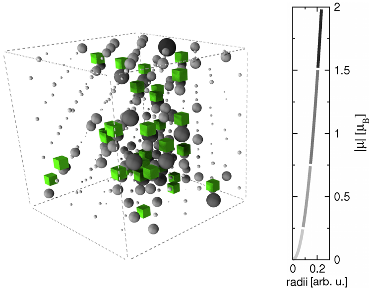
Figure 6.26.: Real space visualization of absolute values of local magnetic moments ( |\mu| ) on N sites (gray), where the color coding and radius of the spheres corresponds to the size of magnetic moment (see legend). Green boxes illustrate V_{\text{Ga}} .
