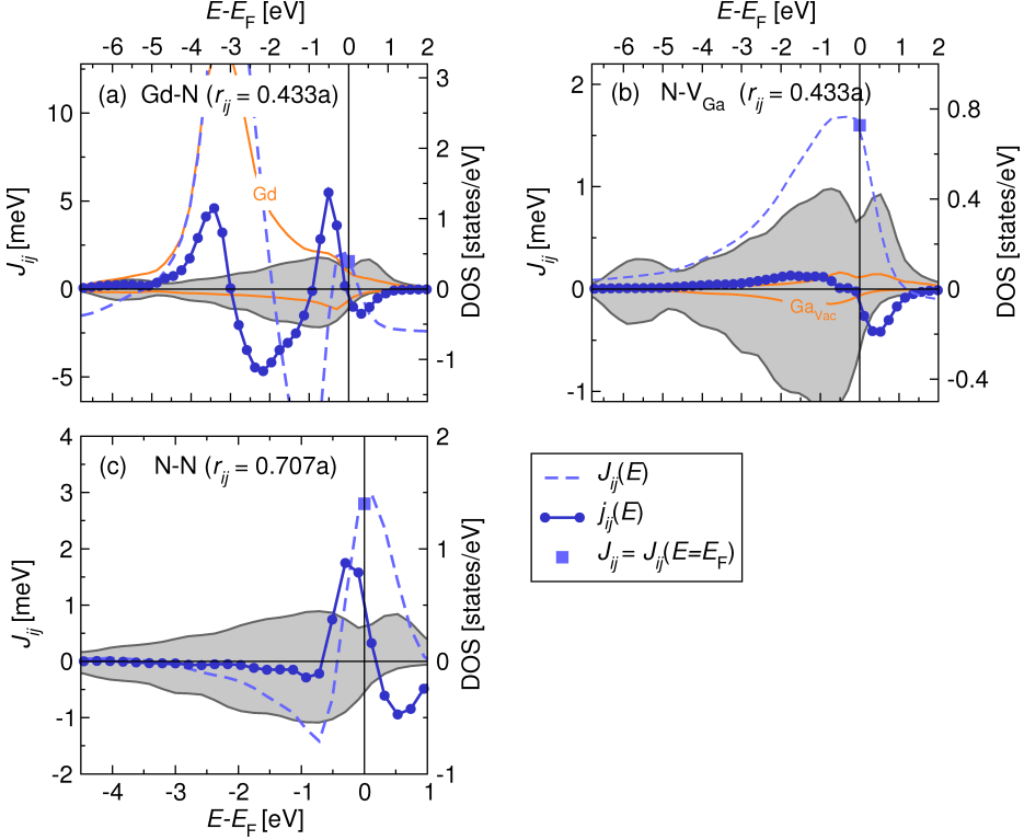
Figure 6.28.: Energy resolved mean exchange interactions j_{ij}(E) , its integration up to E , J_{ij}(E) and its final value J_{ij} for interactions to or from N sites with n_{\text{Vac}} = 1 in \text{Ga}_{220}\text{N}_{256}\text{Gd}_4 . For the sake of comparison the mean DOS of N with n_{\text{Vac}} = 1 is displayed as gray shaded area in (a)-(c). Additionally, in (a) and (b) the mean DOS of Gd and \text{V}_{\text{Ga}} is shown in orange lines. All quantities have been obtained with a temperature-broadening of 700 K and 250 energy integration points.
