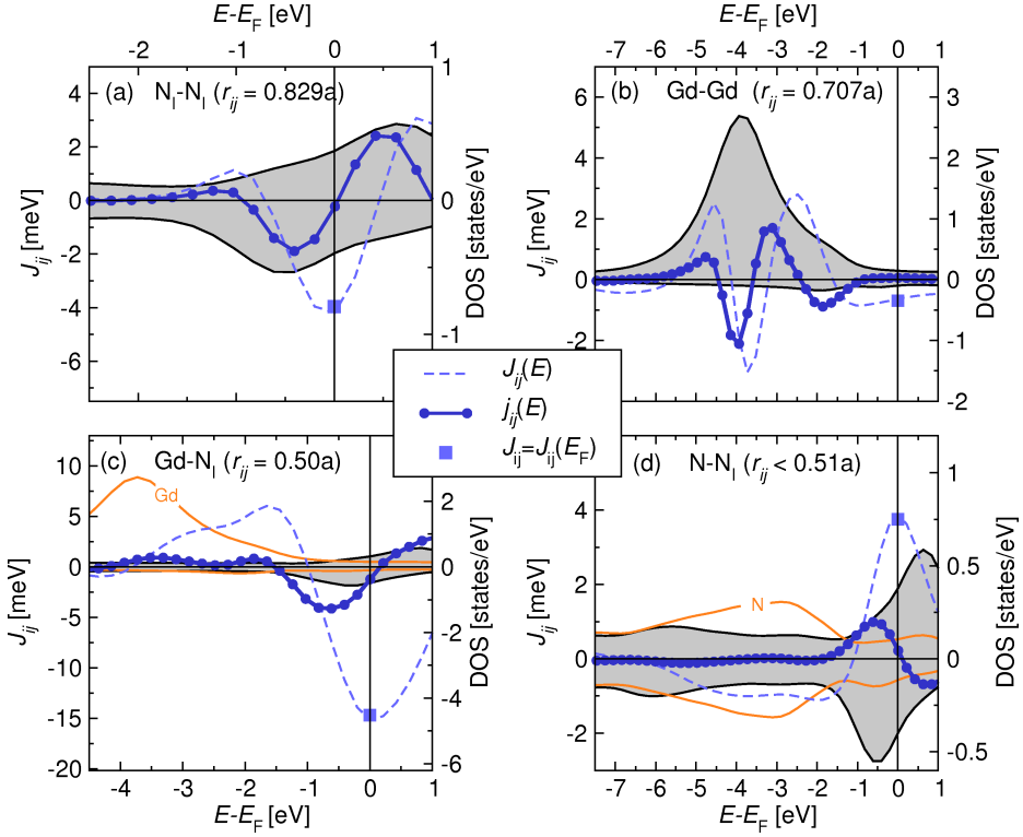
Figure 6.15.: Mean energy-resolved exchange interaction ( j_{ij}(E) ) and mean energy-resolved integrated exchange interaction ( J_{ij}(E) ) at selected interatomic distances r_{ij} for N_1 - N_1 (a), Gd - Gd (b), Gd - N_1 (c), and N_1 - N (d). In all panels the mean local density of states (DOS) of the interacting sites is shown as gray-shaded area, where the minority and majority spin channels are represented by negative and positive DOS values, respectively. In (c) and (d) two different sites are interacting and the DOS of the second component Gd in (c) and N_1 in (d) is displayed in orange lines.
