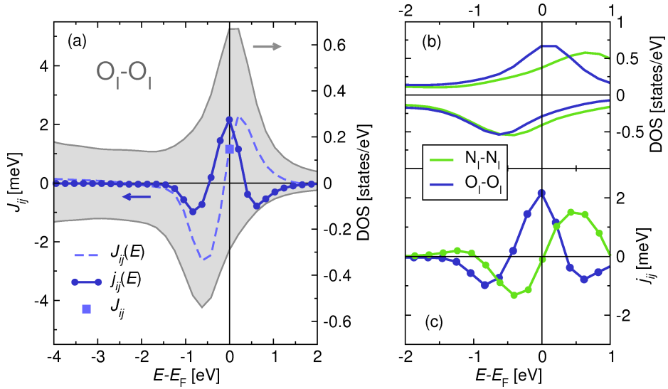
Figure 6.20.: (a) Mean local density of states on O_I sites versus the mean energy-resolved exchange interaction amongst O_I ( O_I-O_I ) j_{ij}(E) , and its mean energy resolved integrated exchange interaction J_{ij}(E) . The square shows the mean exchange coupling constant J_{ij} = J_{ij}(E_F) . All values represent the coupling at a distance r_{ij} = 0.829a in Ga_{256}N_{256}Gd_3O_{1,20} . In (b) the mean LDOS and j_{ij}(E) of O_I and O_I-O_I is shown in comparison to the mean LDOS and j_{ij}(E) of N_I and N_I-N_I for the same interatomic distance.
