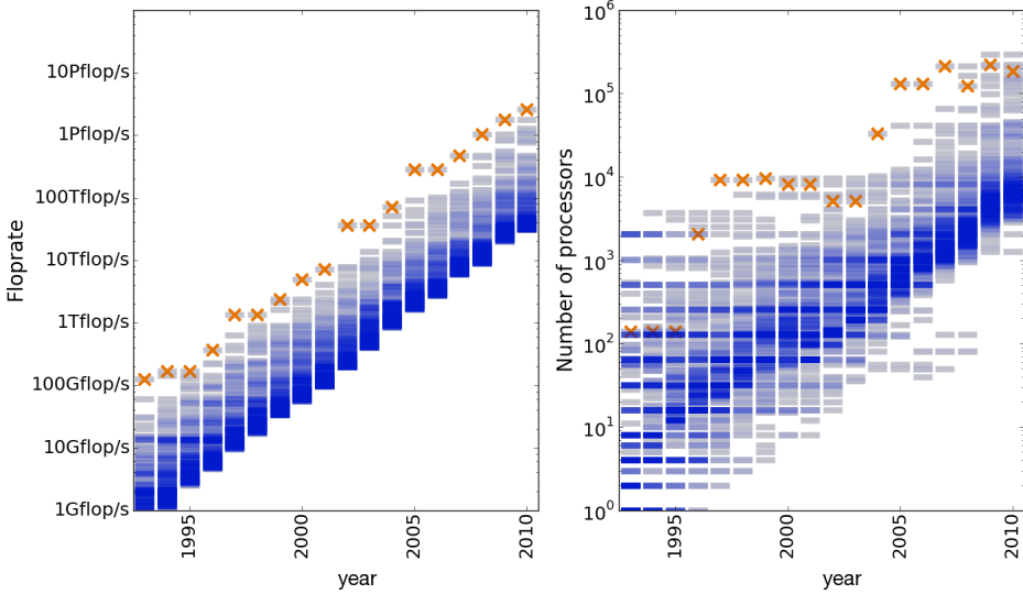
Figure 4.1.: Benchmark flop-rate (left) [81] and number of processors (right) of the 500 fastest supercomputers worldwide. For each of those computers a transparent blue bar visualizes its key properties – accordingly dark blue regions correspond to multiple computers with similar flop-rate or number of processors. The fastest computer with respect to flop-rate is highlighted in yellow. All raw data are taken from [15].
