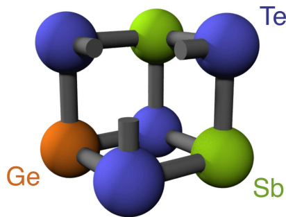
Figure 7.1.: Schematical visualization of \text{Ge}_1\text{Sb}_2\text{Te}_4 in the rocksalt phase. The broken bonds represent the direction to the vacancy.
