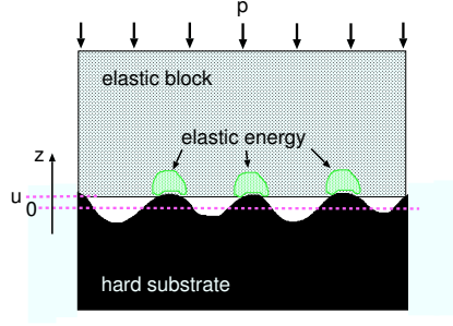
Figure 3: An elastic block squeezed against a rigid rough substrate. The separation between the average plane of the substrate and the average plane of the lower surface of the block is denoted by u . Elastic energy is stored in the block in the vicinity of the asperity contact regions.
