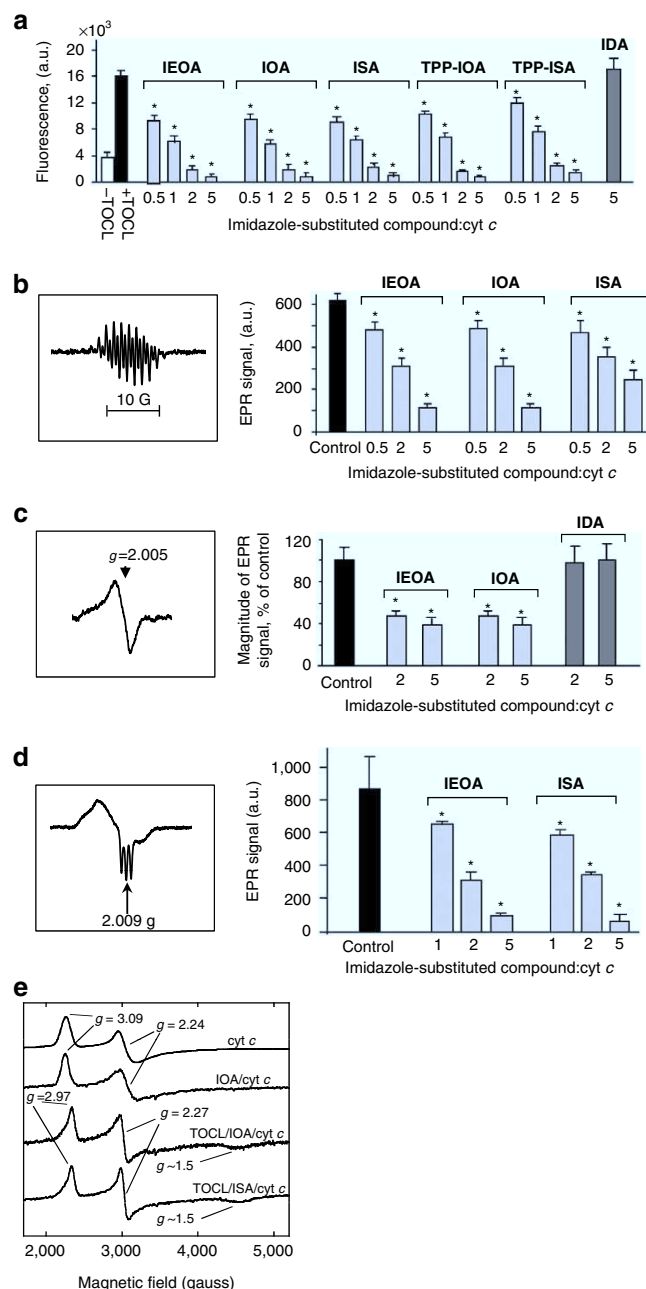
Figure 3 | Inhibition of peroxidase activity of cyt c/TOCL complexes. (a) Assessments of peroxidase activity of cyt c/TOCL by \text{H}_2\text{O}_2 -induced oxidation of Amplex Red to resorufin. Data are means \pm s.d., n = 4 , *P < 0.01 (Student's t -test) versus control (TOCL/cyt c/ \text{H}_2\text{O}_2 with no ISA or IOA or IEOA or TPP-IOA or TPP-ISA added). (b) A typical EPR spectrum of etoposide phenoxyl radicals (left panel). Assessments of peroxidase activity of cyt c/TOCL by \text{H}_2\text{O}_2 -induced oxidation of etoposide using EPR spectroscopy (right panel). (c) A typical low-temperature EPR spectrum of protein-immobilized (tyrosine) radicals (left panel). Assessments of protein-immobilized (tyrosine) radicals by low-temperature (77 K) EPR spectroscopy (right panel). (d) ISA and IEOA limit accessibility of haem to small molecules. A typical low-temperature (77 K) EPR spectrum of cyt c/TOCL complexes in the presence of Angeli's salt (left panel). Effects of ISA and IEOA on haem-nitrosylation of cyt c/TOCL induced by nitroxyl ( \text{HNO} ) generated from Angeli's salt (right panel). Data are means \pm s.d., n = 3 , *P < 0.05 versus control (no ISA and IEOA added). (e) Liquid-He EPR evidence for ligation change in cyt c haem-iron. X-band liquid-He (20 K) EPR spectra of cyt c.
