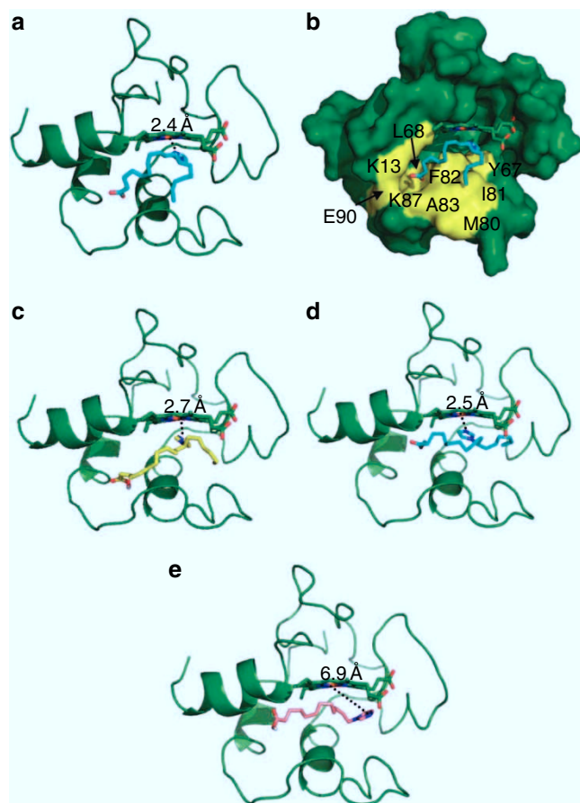
Figure 2 | Modelling of the binding of imidazole substituted fatty acids. (a,b) IOA, (c) ISA, (d) IEOA, and (e) IDA. Cyt c is coloured in green and represented as cartoon in (a,c,d,e) and as surface in (b). IOA, IEOA, ISA, TPP-IOA, TPP-ISA, IDA and haem are represented as sticks. IOA and IEOA are coloured in cyan; ISA is coloured in yellow and IDA is coloured in wheat. The hydrophobic surface corresponding to the predicted IOA binding site is coloured in yellow (b).
