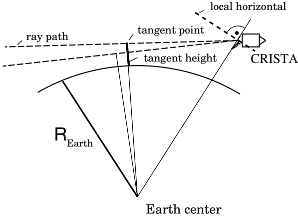
Figure 1. Measuring geometry of the limb sounder. Two rays with different tangent heights are shown. These are obtained by tilting the primary mirror of the instrument.
