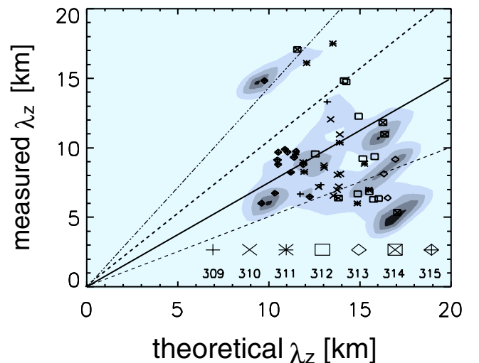
Figure 18. As for Figure 17, but for 50°S–57°S. The solid line indicates the expectations for wave fronts at an angle \Phi = 40^\circ to the mean background wind. Most points cluster around the solid line inside the error limits (dashed lines). The dashed-dotted line indicates \lambda_{z,2D} plus the estimated precision uncertainty of CRISTA. For details, see text.
