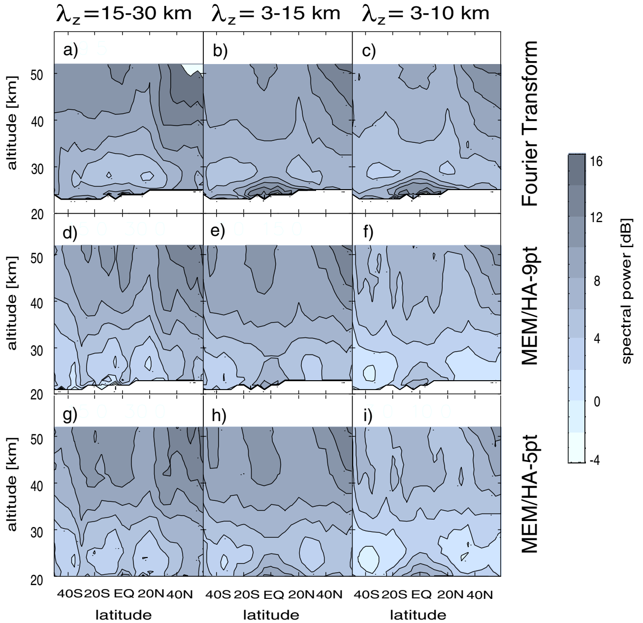
Figure 13. Comparison of zonal mean spectral power in CRISTA residual temperatures using FT (upper row) and MEM/HA on a 9 point (middle row) and 5 point (lowermost row) sliding window for different wavelength ranges (different columns). In general, the agreement is good, but the MEM/HA provides better altitude resolution and thus reproduces the tropical maximum at more realistic altitudes (compare also Figure 12; for details, see text).
