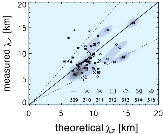
Figure 17. Scatterplot of measured versus theoretical vertical wavelength in the area 42°S–50°S. Symbols show data from different days, from day 309 (5 November) to day 315 (11 November). Almost all the data points lie within the error bars (dashed lines). The shading indicates amplitude-weighted point density. For details, see text.
