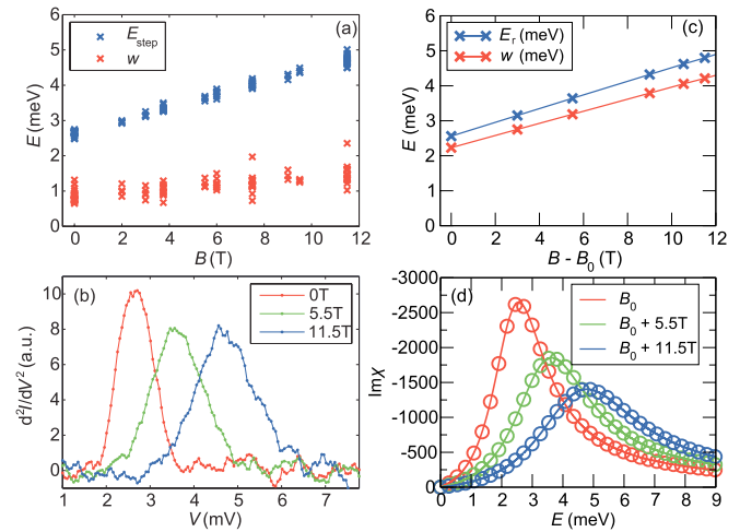
FIG. 2. (Color online) (a) Fitted step energy E_{\text{step}} and step width w (FWHM) of the inelastic step on the positive-voltage side of the ISTS spectra taken on 17 different Fe atoms as a function of magnetic field B . (b) Numerical derivative of the positive-bias part of the spectra used in Fig. 1(a). (c) Calculated magnetic field dependency of the resonance energy E_r and of the linewidth w . (d) Examples of computed density of magnetization excitations for an Fe adatom on Ag(111).
