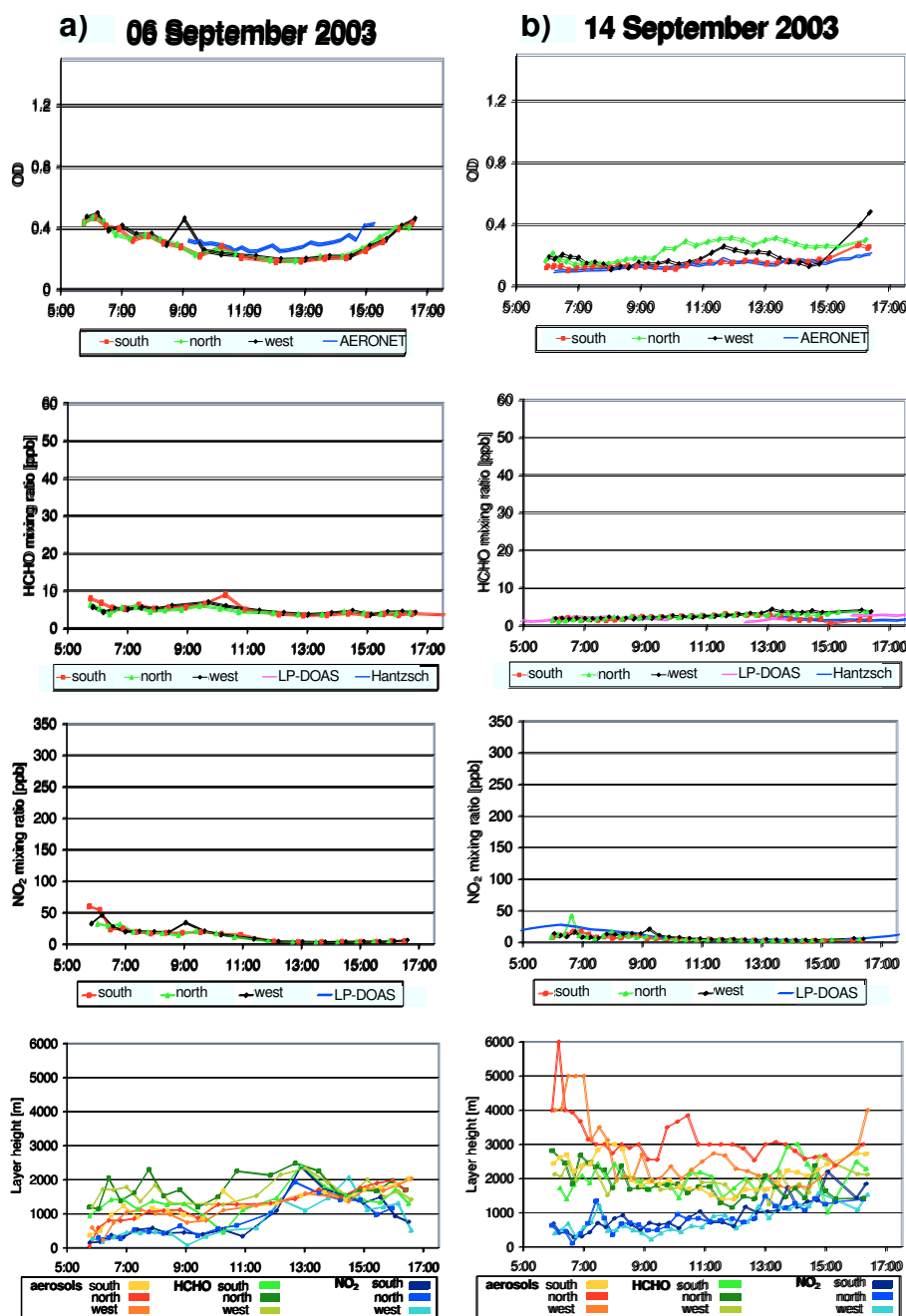
Fig. 15. Retrieval results of the AOD, mixing ratios of HCHO and NO 2 , and layer heights from individual elevation sequences for selected days. Also the results for the LP-DOAS and Hantzschi instrument and the AERONET AOD (at Ispra) are shown for comparison.
