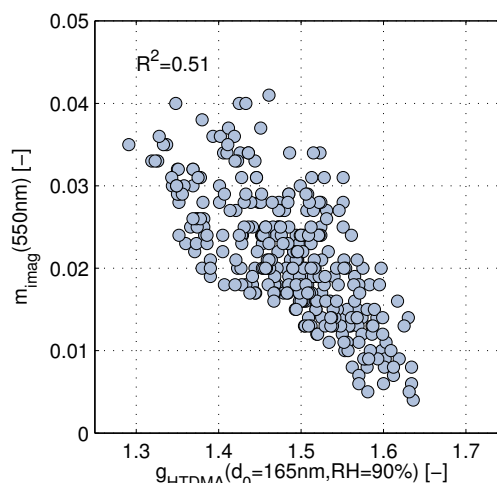
Fig. 4. Retrieved imaginary part of the complex refractive index versus the hygroscopic growth factor measured by the H-TDMA (at d_0 = 165 \text{ nm} and RH=90%).
