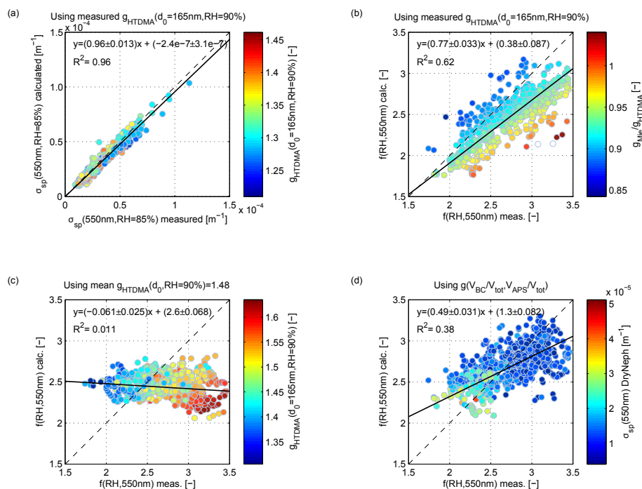
Fig. 5. Panel (a) Scattering coefficient \sigma_{sp} calculated vs. measured using the hygroscopic growth factor measured by the H-TDMA. Panel (b)–(d) Scattering enhancement factor f(RH = 85\%, 550 \text{ nm}) calculated vs. measured values. Panel (b) The measured hygroscopic growth factor of the H-TDMA (dry diameter d_0 = 165 \text{ nm} ) has been used for the calculation, the color code denotes the ratio of g_{Mie}/g_{HTDMA} . Panel (c) A fixed value of g(d_0 RH = 90\%) = 1.48 (mean for that period) has been used for the calculation. Panel (d) An empirical relation of g(V_{BC}/V_{tot}, V_{APS}/V_{tot}) has been used for the calculation of f(RH) . All values are shown at RH = 85\% . The solid black line represents a bivariate linear regression including weights (with calculated uncertainty of slope and intercept). The 1:1-line is shown as a dashed line.
