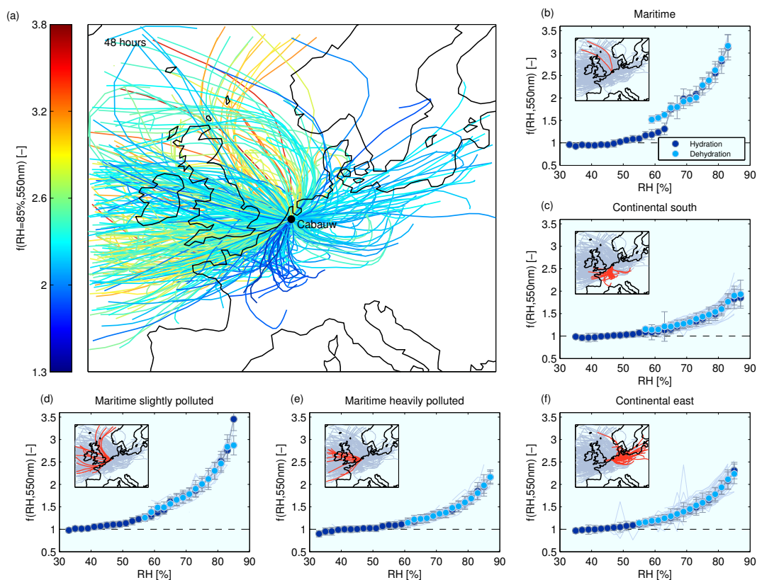
Fig. 2. Panel (a) FLEXTRA trajectories (48 h backward calculation) of air parcels arriving at Cabauw. The trajectories are color coded with the mean aerosol scattering enhancement f(\text{RH}=85\%, 550\text{ nm}) measured at the site. Panels (b)–(f) Example humidograms classified by the origin of the air masses. Dark blue circles denote averages of f(\text{RH}) for the hydration branch of the humidogram, while light blue circles are averages of the dehydration branch (2% RH bins). Underlined in grey are the individual humidograms of each trajectory. Error bars denote the standard deviation.
