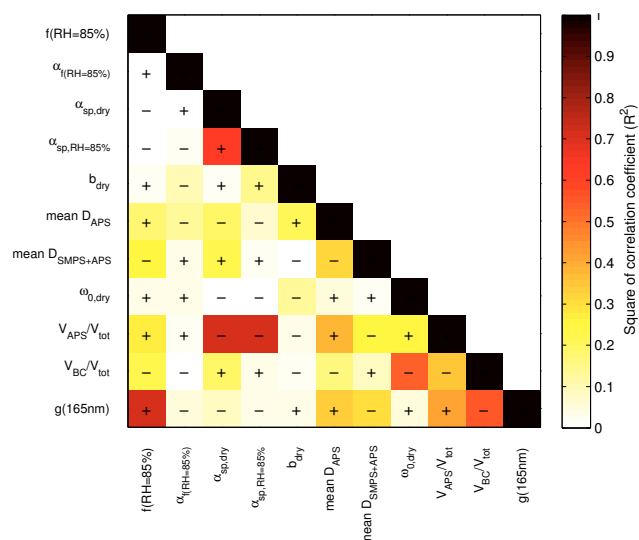
Fig. 3. Correlation plot of all intensive aerosol parameters measured in-situ at the Cabauw tower. f(\text{RH}=85\%, 550 \text{ nm}) : scattering enhancement factor; \alpha_f(\text{RH}) : Ångström exponent of f(\text{RH}=85\%, 550 \text{ nm}) ; \alpha_{\text{sp,dry}} : Ångström exponent of scattering coefficient at low RH; \alpha_{\text{sp,RH}=85\%} : Ångström exponent of scattering coefficient at RH=85%; b_{\text{dry}} : backscatter fraction (at \lambda = 550 \text{ nm} ) at low RH; D_{\text{APS}} : mean (dry) diameter of APS size distribution measurement; D_{\text{SMPS}} : mean (dry) diameter of SMPS size distribution measurement; \omega_{0,\text{dry}} : single scattering albedo at low RH (at \lambda = 550 \text{ nm} ); V_{\text{APS}}/V_{\text{tot}} : coarse mode fraction measured by APS and SMPS; V_{\text{BC}}/V_{\text{tot}} : black carbon volume fraction measured by MAAP, SMPS, and APS; g(\text{RH}=90\%, 165 \text{ nm}) : hygroscopic growth factor measured at the dry diameter d_0 = 165 \text{ nm} and at RH=90% by the H-TDMA. Plus and minus signs indicate the slope of the regression line.
