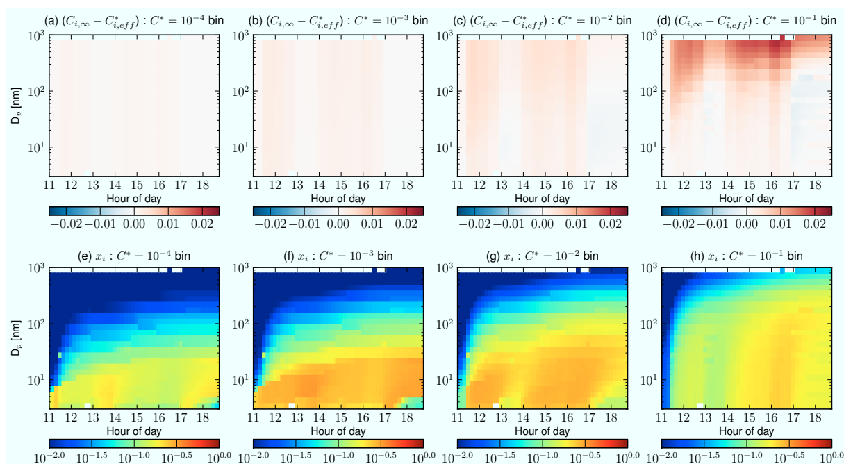
Fig. 5. Demonstration of how the equilibrium effect can inhibit ultrafine particle growth for Hyytiälä on 10 April 2007. Panels (a–d) show the condensational driving force ( C_{i,\infty} - C_{i,eff}^* ) [ \mu\text{g m}^{-3} ] as a function of aerosol size and time for the C^* = 10^{-4} , 10^{-3} , 10^{-2} and 10^{-1} [ \mu\text{g m}^{-3} ] volatility bins for the simulation where pre-existing SOA has C^* = 10^{-5} [ \mu\text{g m}^{-3} ], freshly formed SOA has a LOGTRI volatility distribution, SOA does not readily partition into sulfate and water, the surface tension is 0 \text{ N m}^{-1} , and the accommodation coefficient is 1. Panels (e–h) show the mass mixing ratio ( x_i , note that the volatility basis set uses mass mixing ratios rather than molar mixing ratios) as a function of aerosol size and time for the same simulation.
