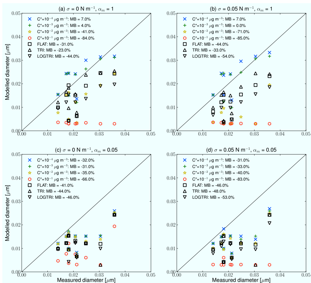
Fig. 4. Comparison of the simulated diameter to measured diameter of the nucleation mode after SOA condensation has stopped for the 7 events at Hyttälä and Egbert. All simulations assumed that pre-existing organics have C^* = 10^{-5} \mu\text{g m}^{-3} and assumed that organics do not partition into sulfate and water. In each panel, different cases regarding the volatility distribution of organics are marked by different colors and symbol shapes. Panel (a) assumed surface tension is 0 \text{ N m}^{-1} and accommodation coefficient is 1. Panel (b) assumed surface tension is 0.05 \text{ N m}^{-1} and accommodation coefficient is 1. Panel (c) assumed surface tension is 0 \text{ N m}^{-1} and accommodation coefficient is 0.05. Panel (d) assumed surface tension is 0.05 \text{ N m}^{-1} and accommodation coefficient is 0.05. MB denotes the mean bias across the 9 events.
