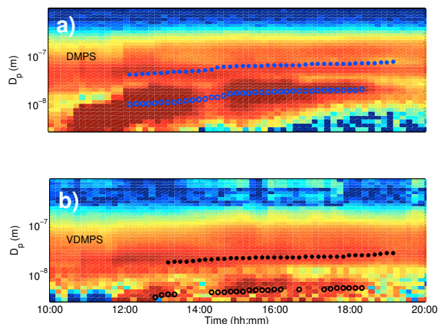
Fig. 2. Timeseries of the aerosol size distribution with time measured by the (a) DMPS and (b) VDMPS on 10 April 2007 in Hyytiälä. Aerosols in VDMPS were heated to 280^\circ\text{C} for 1 s before measurement. The blue and black markers denote the geometric number-mean diameters of the Aitken and nucleation modes for each size scan. These number-mean diameters are averaged over the time of the nucleation event and used as inputs to the C^* fit in the kinetic evaporation model.
