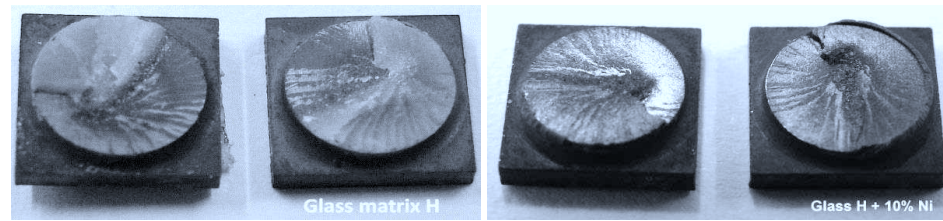
Fig. 59 Fracture of hour-glass samples after the torsion test measurement. All the composite sealants showed similar fracture patterns.
