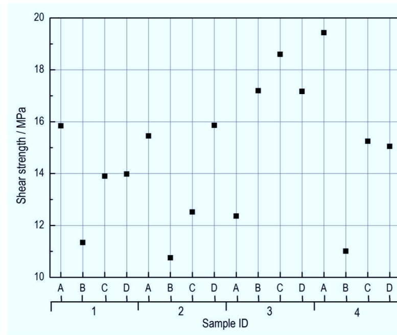
Fig. 45 Shear strength results attained with the first sample concept (Fig. 44a). The variation in shear strength could be the result of pre-damage caused by sample A to sample B, C, or D
