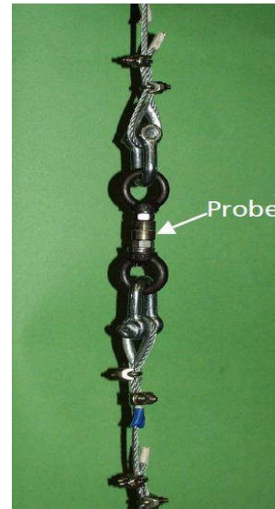
Fig. 16 Joined samples in the tensile strength measurement set-up [Sch 2002b]
