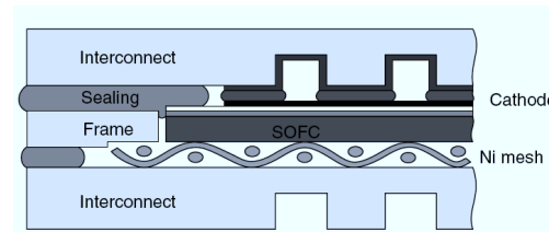
Fig. 1 Schematic presentation of a repeating unit of a planar SOFC with a rigid glass-ceramic seal [Buc 2010]
