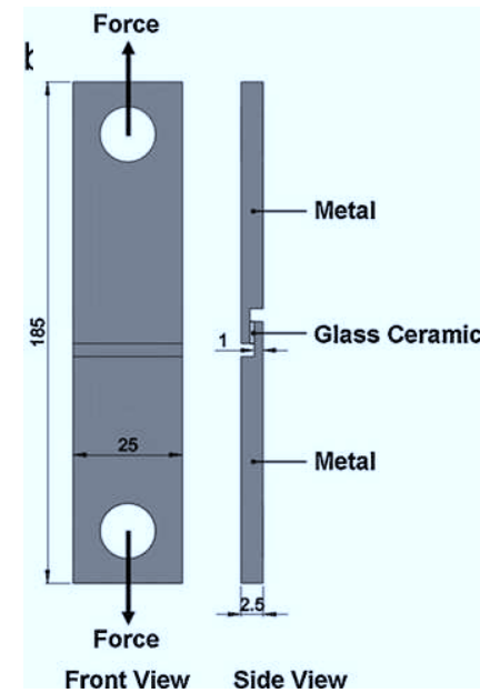
Fig. 13 Joint specimen for shear test, dimensions in mm [Lin 2012]
