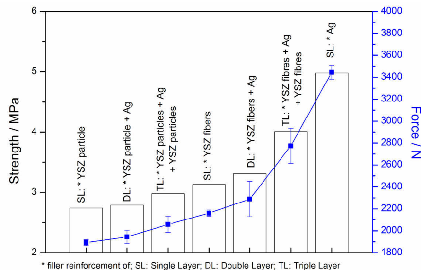
Fig. 55 Strength comparison of single-layer and multilayer composites
