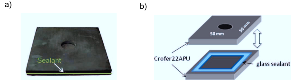
Fig. 20 a) Sandwich sample formed of two Crofer22APU plates of 50 x 50 mm 2 dimension joined by glass-ceramic sealant. b) Schematic view of a sandwich sample open with the applied sealant
