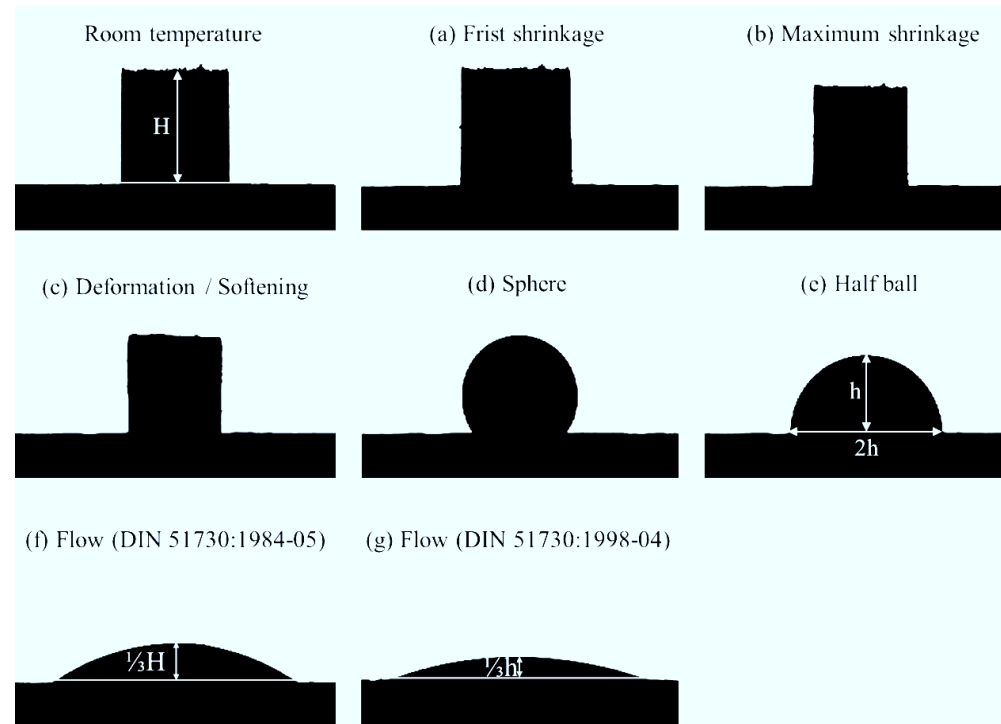
Fig. 18 Geometric shape corresponding to each fixed viscosity point [Pas 2001]; [Pas 2005]; [DIN 1984]; [DIN 1998]
