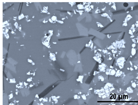
Fig. 39 Good dispersion of 20 wt.-% CGO particles in glass matrix 87. No interface or reaction zone formed between the filler and glass
