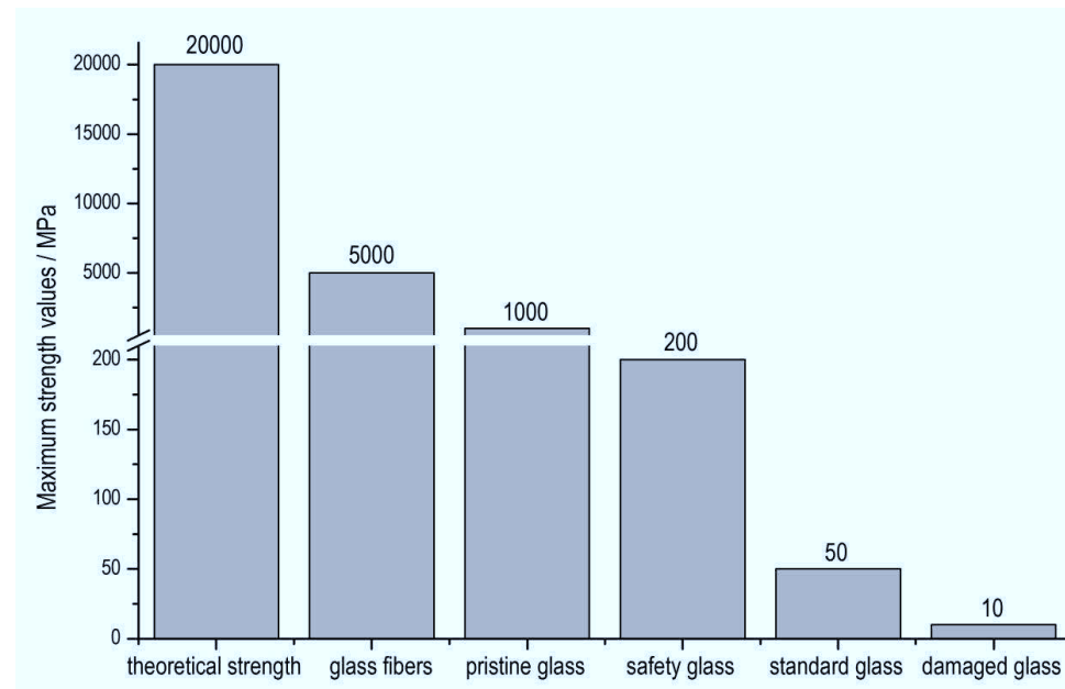
Fig. 5 Typical maximum strength of glasses
