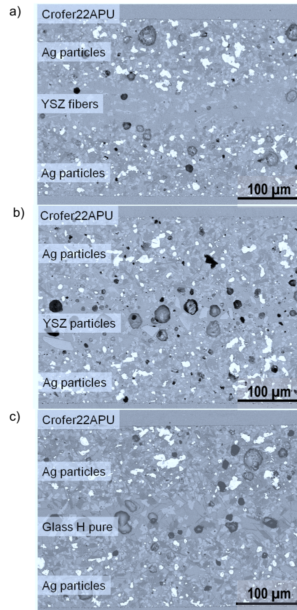
Fig. 50 Triple-layered sandwich samples with outer layers reinforced with silver particles, and inner layer filled with: a) YSZ fibers; b) YSZ particles; c) pure glass
