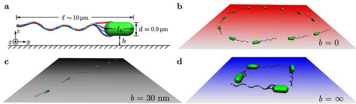
Figure 1 | Swimming bacteria sense the slip of its nearby surface. (a) The model bacterium of length \ell consists of a spherocylindrical body of length \ell_b and diameter d and four helical flagella each turned by a motor torque. The bacterial geometry and flagellar properties are in agreement with experiments of E. coli (Methods and SI). The body the flagellar bundle counter rotate. h is the gap width between the body and the surface. (b) CW, (c) noisy straight, and (d) CCW trajectories from hydrodynamic simulations of a bacterium swimming near homogeneous surfaces with different slip lengths b as indicated.
