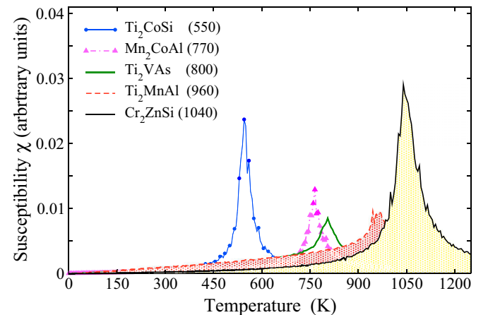
FIG. 6. (Color online) Calculated temperature dependence of the susceptibility for SGSs. The maximum of the susceptibility corresponds to the critical temperature (shown in parentheses in the legends).
