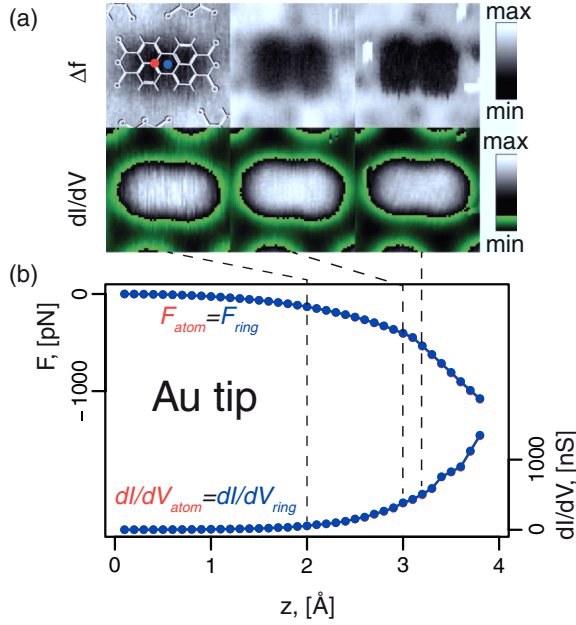
FIG. 1. (Color) (a) 64 \times 64 \text{ pixel} , 13 \times 13 \text{ Å}^2 constant height \Delta f (top) and dI/dV (bottom) images selected from the image sequence measured above the PTCDA molecule adsorbed on Au(111) with the clean Au tip. Tunneling bias: V = -12 \text{ mV} . The chemical structure formula of PTCDA is shown, red and blue circles mark the positions at which F(z) and dI/dV(z) were evaluated. The used color scales are shown next to the respective groups of images. The two-color scale was used for better representation of the large dynamic range in the dI/dV images. For the \Delta f images in the left, middle, and right panels the (\Delta f_{\min}, \Delta f_{\max}) of the corresponding scales are (-26 \text{ Hz}, -23 \text{ Hz}) , (-45 \text{ Hz}, -32 \text{ Hz}) , and (-85 \text{ Hz}, -50 \text{ Hz}) . For the dI/dV images the (dI/dV_{\min}, dI/dV_{\max}) of the corresponding scales are (10 \text{ nS}, 77 \text{ nS}) , (50 \text{ nS}, 416 \text{ nS}) , and (66 \text{ nS}, 562 \text{ nS}) . (b) F(z) (top) and dI/dV(z) (bottom) spectra extracted from the image series shown in Fig. 1(a). 8 The blue spectra were obtained above the center of the carbon ring [blue circle in Fig. 1(a)]; the red spectra, at the carbon atom [red circle in Fig. 1(a)]. Note that in the case of the clean Au tip the red and the blue spectra coincide. The F scale is defined such that a negative (positive) value corresponds to an attractive (repulsive) force. For the definition of the z scale see Ref. 7. The dashed lines mark the z values at which the images from Fig. 1(a) were measured.
