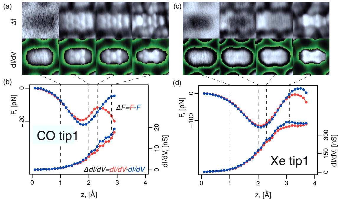
FIG. 2. (Color) In (a) and (c), 64 \times 64 pixel, 13 \times 13 Å constant height \Delta f (top) and dI/dV (bottom) images selected from the image sequences measured above the PTCDA molecule adsorbed on Au(111) with the (a) CO and (c) Xe tips are shown. Tunneling bias: V = -12 mV. For the \Delta f images the (\Delta f_{\min}, \Delta f_{\max}) of the used color scales are (from left to right) (-11 Hz, -7 Hz), (-13 Hz, 9 Hz), (-12 Hz, 17 Hz), (-14 Hz, 30 Hz) for CO; and (-6 Hz, -4 Hz), (-11 Hz, -7 Hz), (-11 Hz, 2 Hz), (-6 Hz, 20 Hz) for Xe images. (dI/dV_{\min}, dI/dV_{\max}) from left to right are (0.1 nS, 2 nS), (2 nS, 21 nS), (2 nS, 29 nS), (4 nS, 42 nS) for CO; and (2 nS, 15 nS), (7 nS, 109 nS), (9 nS, 176 nS), (19 nS, 374 nS) for Xe. In (b) and (d), F(z) (top) and dI/dV(z) (bottom) spectra extracted from the series of images measured with the (b) CO and (d) Xe tips are displayed. 8 The color coding of the spectra is the same as in Fig. 1(b). The F scale is defined similarly to Fig. 1(b). For the definition of the z scale, see Ref. 7. The dashed lines mark the z values at which the images from (a) and (c) were measured.
