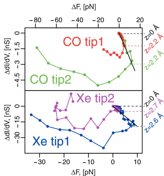
FIG. 3. (Color) Conductance response \Delta dI/dV vs the applied force \Delta F(z) . The upper (lower) panel shows spectra measured with two different CO (Xe) tips. The regime in which the response of conductance is linear is indicated by the black fitted lines. The distance at which each tip starts to deviate from the linear response regime is marked on the right.
