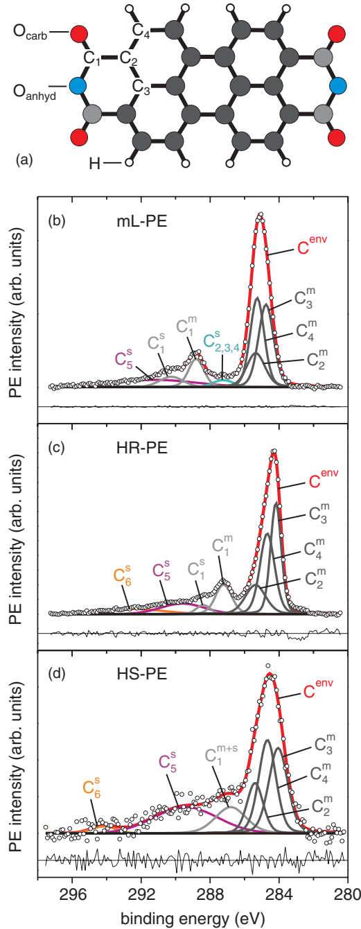
FIG. 6. (Color) (a) PTCDA molecule. (b) C1s mL-PE spectrum (open circles) of a PTCDA/Ag(100) multilayer ( \approx 40 ML), measured at the beamline ID32 (ESRF, Grenoble). (c) Sum of 26 C1s HR-PE spectra (open circles) of submonolayer PTCDA/Ag(110), measured with a laboratory source. (d) C1s HS-PE spectrum (open circles) of submonolayer PTCDA/Ag(110), measured at the beamline ID32 (ESRF, Grenoble). The acquisition settings of spectra (b)–(d) are reported in Sec. II B1. Displayed are PE intensity (open circles); C^{env} (thick red line); C_2^m , C_3^m , C_4^m (dark gray lines); C_1^m , C_1^s , C_1^{m+s} (light gray lines); C_{2,3,4}^s (cyan line); C_5^s (magenta line); C_6^s (orange line); background (straight black line); and residuals (black line below each spectrum).
