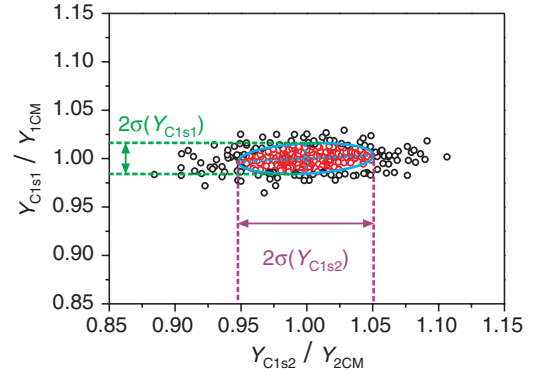
FIG. 4. (Color) Plot of the (Y_{\text{C1s1}}, Y_{\text{C1s2}})^{\text{MC}} distribution resulting from the fit of 400 Monte Carlo simulations of the spectrum in Fig. 3. The blue ellipse contains all points of the distribution that lie within the confidence region (68.3% of all points). The center of the ellipse is the center of mass (CM) of the distribution. The principal axes are indicated by dotted blue lines. Points within the confidence region are represented by red open circles; those outside are marked by black open circles. The confidence interval of the two fitting parameters 2\sigma(Y_{\text{C1s1}}) and 2\sigma(Y_{\text{C1s2}}) are marked by dashed lines. Note that the axes are normalized to the PE yields of the center of mass (Y_{1\text{CM}}, Y_{2\text{CM}}) .
