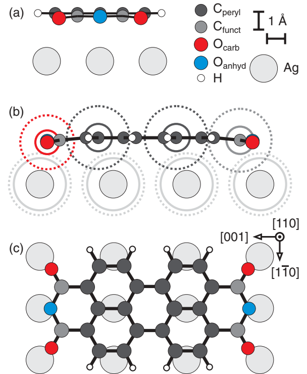
FIG. 9. (Color) (a) Side view (along the long molecular axis) of PTCDA/Ag(110). (b) Side view (along the short molecular axis) of PTCDA/Ag(110). (c) Top view of PTCDA/Ag(110). Solid circles indicate the atomic positions. In panel (b), solid lines indicate covalent radii (Ref. 54) ( r_{\text{cov}}^C = 0.73 Å, r_{\text{cov}}^O = 0.66 Å, r_{\text{cov}}^{\text{Ag}} = 1.45 Å) and dotted lines indicate van der Waals radii (Ref. 55) ( r_{\text{vdW}}^C = 1.75 Å, r_{\text{vdW}}^O = 1.50 Å, r_{\text{vdW}}^{\text{Ag}} = 1.72 Å).
