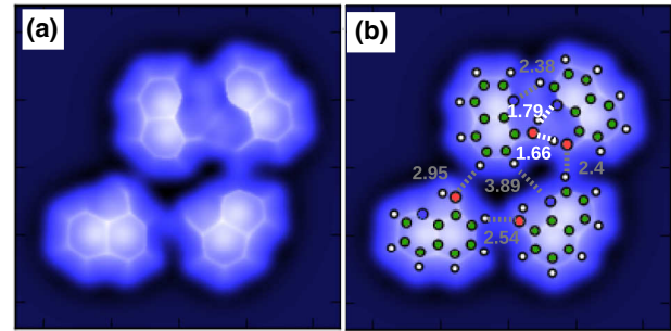
FIG. 5. (Color online) Sharp intermolecular contrast and hydrogen bonds, part I. (a) A simulated AFM image for a 8-hydroxyquinoline tetramer with CO probe particle (tip-sample distance 7.4 Å). The sharp lines in intermolecular regions agree very well with the contrast reported in Fig. 2d of Ref. [17]. (b) Same image as in panel (a), but with a schematic overlay of the molecular structure, with atoms discriminated by colors (white: hydrogen; green: carbon; blue: nitrogen; red: oxygen) and hydrogen bonds (short and strong hydrogen bonds: white; weaker hydrogen bonds: gray). Numbers indicate bond lengths in Å. The image color scale is rescaled by maximum and minimum values of \Delta f to provide best contrast.
