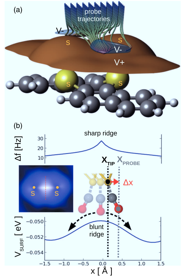
FIG. 3. (Color online) Origin of sharp lines in AFM images. (a) DBTH molecule (sulfur atoms in yellow, carbon atoms in dark gray, and hydrogen atoms in light gray), with repulsive potential felt by the probe particle in brown ( V^- ) and attractive basins ( V^+ ) in blue. Probe particle trajectories upon tip approach are also shown. Sulfur-derived hillocks in the repulsive potential are labeled “S.” Between them, a repulsive saddle is formed. (b) Surface potential V_{\text{surf}} (bottom) and AFM frequency shift \Delta f (top) along the central cross section of the repulsive saddle. In the center the relaxation \Delta x of the probe particle towards the position x_{\text{probe}} is shown schematically for a tip position x_{\text{tip}} close to the ridge of the saddle. The mapping of the force at x_{\text{probe}} to the macroscopic tip position x_{\text{tip}} explains the sharpening of the \Delta f curve (“sharp ridge”) even for a smooth saddle in V_{\text{surf}} (“blunt ridge”). The inset shows a simulated AFM image of DBTH in the region of the two sulfur atom, clearly exhibiting the sharp line between the two sulfur atoms.
