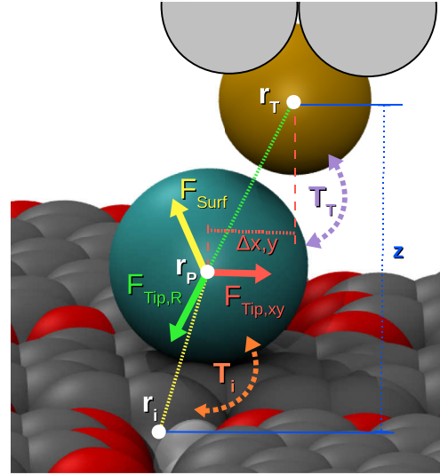
FIG. 1. (Color online) AFM/STM model. Schematic view of the mechanical model of a functionalized tip as employed in this work. The last metal atom of the tip ( tip base ) is shown in sand color, the probe particle in cyan, and the molecular layer ( sample , in the example a herringbone PTCDA layer) in gray (carbon atoms) and red (oxygen atoms). The forces acting on the probe particle are shown in color: radial tip force F_{\text{Tip,R}} (green); lateral tip force F_{\text{Tip,xy}} (red); force F_{\text{Surf}} exerted by atoms of the sample (yellow). Force-determining geometric parameters are shown in the same color as the corresponding forces. The two distinct hopping processes in our STM model are denoted by violet (probe particle tip, T_T ) and orange (probe particle sample, T_i ) color. The reference distance z that is used throughout the paper is shown in blue.
