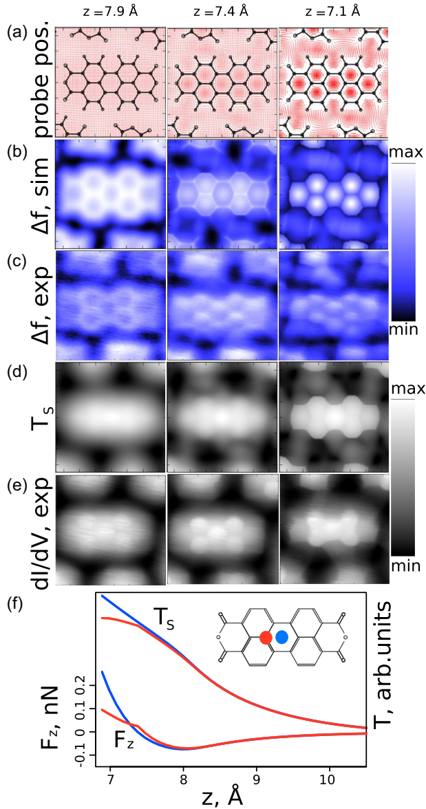
FIG. 2. (Color online) Simulated and experimental high-resolution AFM and STM images. Experimental images have been recorded on PTCDA/Au(111) with a CO probe particle. Simulated images have been obtained with LJ parameters mimicking the oxygen atom of CO. (a) Map of simulated probe particle positions after relaxation. (b) Simulated AFM image (the frequency shift \Delta f is displayed). (c) Experimental AFM images (frequency shift). (d) Simulated STM images (maps of the T_s tunneling process). (e) Experimental STM images (differential conductance). (f) Vertical force F_z (left axis) and tunneling probability T_s (right axis, arbitrary units), both as a function of tip-sample distance z , computed over different sites of the sample as indicated by the red and blue dots in the PTCDA structure formula. Experimental images in panels (c) and (e) are taken from Ref. [9]). All simulated images except (a) are normalized to obtain maximum contrast.
