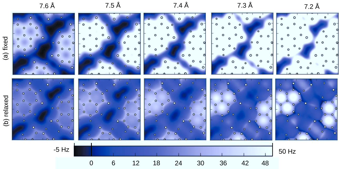
FIG. 6. (Color online) Sharp intermolecular contrast and hydrogen bonds, part II. Simulated AFM images of a monolayer of naphthalene tetracarboxylic diimide (NTCDI) molecules that was studied experimentally by Sweetman et al. in Ref. [23]. (a) Without probe particle relaxation; (b) with probe particle relaxation. The images in panel (b) agree very well with experimental AFM images in Figs. 1b and 1c of Ref. [23].
