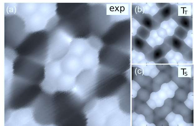
FIG. 4. Intermolecular contrast in high-resolution STM images. (a) Experimental constant height image recorded with a Xe tip over PTCDA/Ag(111). Imaging parameters: area 18 \text{ \AA} \times 18 \text{ \AA} ; V = -4 \text{ mV} . Prior to the imaging the tip was stabilized at I = 0.1 \text{ nA} and V = -350 \text{ mV} ; then the bias was changed to V = -4 \text{ mV} and the tip was moved by 4 \text{ \AA} closer to the surface. (b) Simulated STM image with Xe probe particle ( T_T tunneling channel). (c) Simulated STM image with Xe probe particle ( T_S tunneling channel). Panels (b) and (c) display approximately the same area as panel (a).
