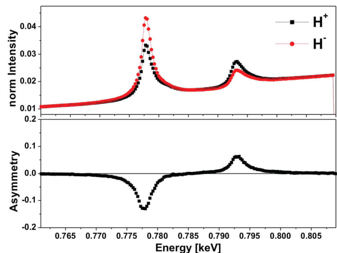
FIG. 7. Top panel: energy scan in reflection geometry near the Co L_3 and L_2 edges taken in positive and negative magnetic fields of 2700 Oe at a temperature of 40 K. The intensity is normalized to the monitor counts. Bottom panel: asymmetry signal of Co derived from the reflectivity data.
