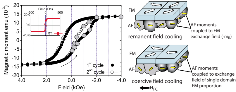
FIG. 1. (Color online) (a) SQUID hysteresis loops of [\text{Co}/\text{CoO}/\text{Au}]_{16} ML during the first (solid symbol) and second field cycles (open symbol) for H_{\text{FC}} = +20 Oe. The loops correspond to a coercive field cooling state after positive saturation at RT and the arrow along the curve indicates the field sweeping direction. The inset shows the hysteresis loop at RT. The gray dots are the points of field along the curve used in neutron measurements. Schematics represent the state of the FM-AFM layer magnetization after being field cooled at remanent cooling field ( -m_R ) and at H_{\text{FC}} \approx H_c .
