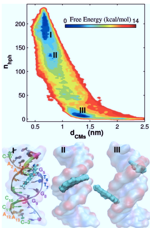
FIG. 4. (Upper panel) Free energy as a function of the two collective variables used in metadynamics, that is, the distance d_{CMs} between the center of mass of the ligand and of the DNA tracts d[GTGG]_2 and the number of hydrophobic contacts n_{hph} between nonpolar carbons on the ligand and on the bases covered by the ligand in the starting structure. (Lower panel) The typical configurations picked in the region as marked in the free energy plot in the upper panel. The two overlapping configurations marked III show two possible configurations in region III .
