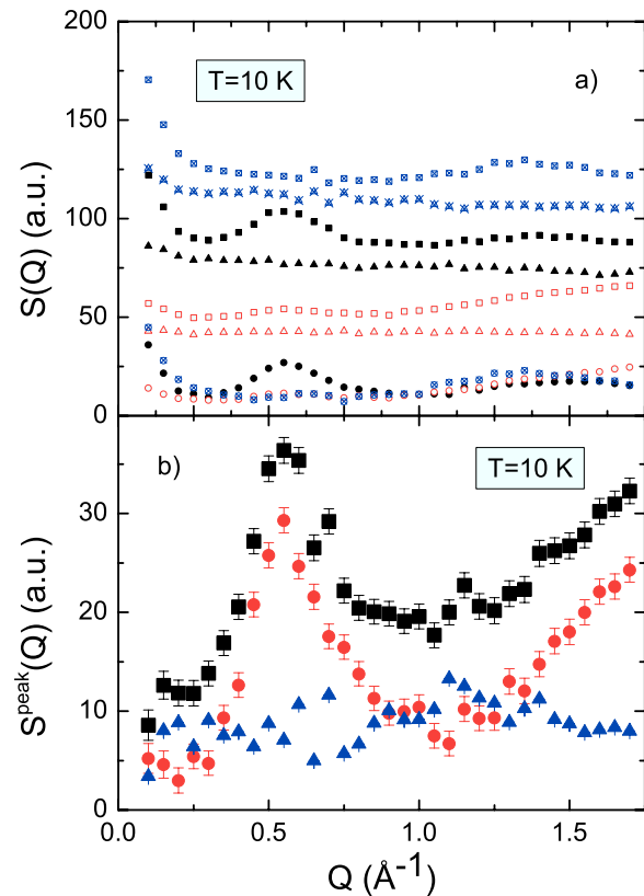
FIG. 8. (a) The structure factor measured by the NCNR NSE spectrometer for C_7H_7D_2N (solid black symbols), for C_7H_2D_7N (open red symbols), and C_7H_9N (starred open blue symbols). Squares, circles, and triangles refer to the total, coherent, and incoherent scattering intensity, respectively. The size of the error bars (not shown) is approximately the same as the size of the symbols. (b) The total (black squares), coherent (red circles), and incoherent (blue triangles) scattering intensity of S^{\text{peak}}(Q) as defined in Eqs. (7)–(9), respectively.
