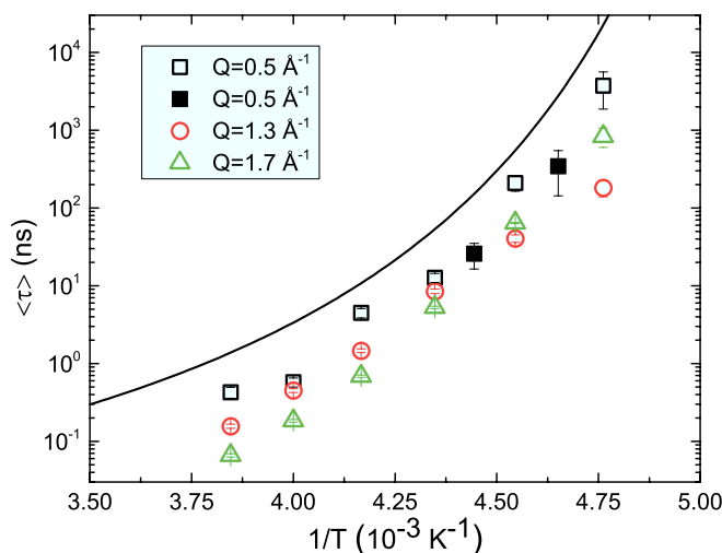
FIG. 6. Arrhenius plot of the average relaxation times \langle \tau \rangle (see Eq. (5)) obtained from the fits of the NSE data using a stretched exponential function, Eq. (3), fixing the stretching exponent to its temperature averaged value. The open symbols refer to the results obtained using the NCNR NSE and the closed squares refers to the results from the SNS NSE. The continuous black line shows the temperature dependence of the viscosity, 13 arbitrarily scaled to allow a comparison to the \langle \tau \rangle values.
