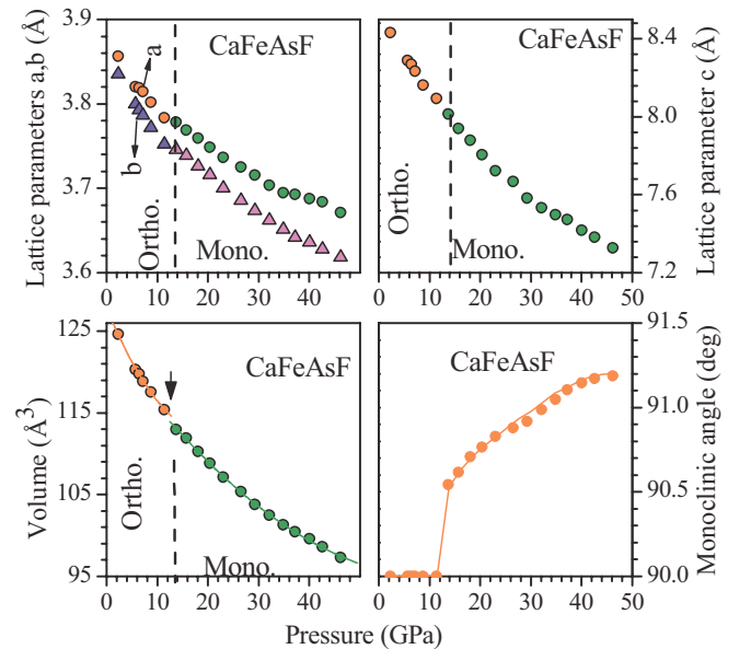
FIG. 9. (Color online) Pressure dependence of the structural parameters (lattice parameters, volume, and monoclinic angle) of CaFeAsF at 40 K as obtained after Rietveld analyses of data with increasing pressure. For the sake of comparison, lattice parameters along [100], [010] and volume of the orthorhombic phase are divided by \sqrt{2} and 2, respectively, and lattice parameters of monoclinic phases are plotted in a standard (cab: P12/n1 ) setting. Errors are within symbol size.
