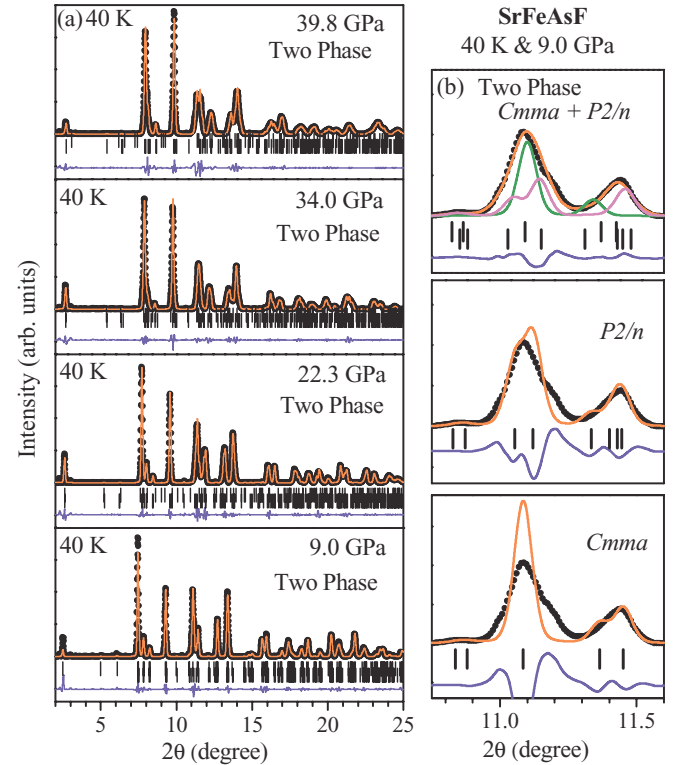
FIG. 8. (Color online) (a) Observed (solid black circles), calculated (continuous red/dark gray line), and difference (bottom blue/medium gray line) profiles obtained after the Rietveld refinement of SrFeAsF at selected pressures and 40 K. The diffraction profiles at 9.0, 22.3, 34.0, and 39.8 GPa are refined using a combination of orthorhombic ( Cmma ) and monoclinic ( P2/n ) phases. Upper and lower vertical tick marks above the difference profiles indicate peak positions of orthorhombic ( Cmma ) and monoclinic ( P2/n ) phases, respectively. (b) The refinement of the diffraction pattern at 9.0 GPa and 40 K with an orthorhombic phase (space group Cmma ), a monoclinic ( P2/n ) phase, and a combination of orthorhombic (space group Cmma ) and monoclinic ( P2/n ) phases.
