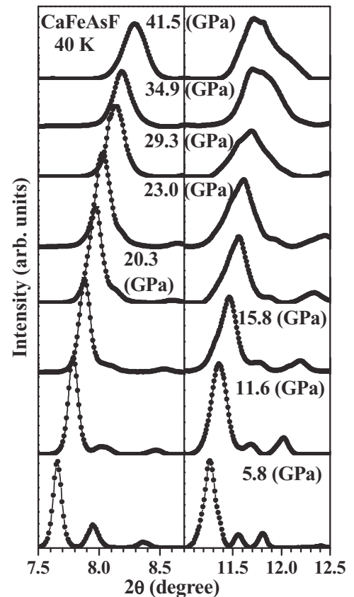
FIG. 3. Evolution of the powder-synchrotron x-ray diffraction patterns of CaFeAsF at 40 K and selected pressure.
