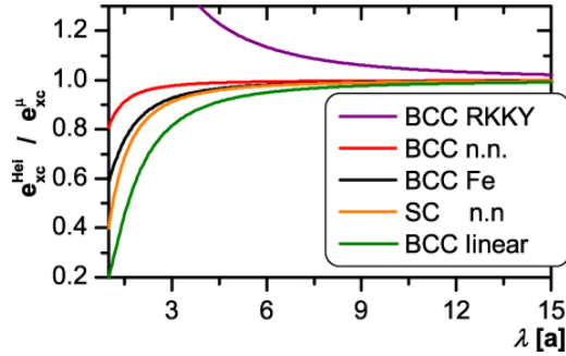
Figure 6: The micromagnetic approximation for the exchange energy e_{xc}^{\mu} according to eq. (7) ceases to be valid for strongly inhomogeneous structures. The Heisenberg term, which can take different forms depending on the number of interacting atoms and the value of the exchange integral, assumes in any case a finite value, whereas the continuum expression diverges as \lambda goes to zero. Well before \lambda = a poses a natural limit for the largest inhomogeneity in the Heisenberg model, the equations yield significantly different results. The materials are chosen according to [35].
