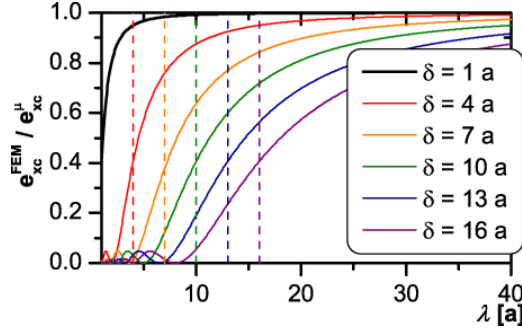
Figure 5: The ratio of the computed micromagnetic exchange energy e_{xc}^{FEM}(\lambda, \delta) and the corresponding analytic value e_{xc}^{\mu}(\lambda) reaches very low values for small \lambda and large discretization cell size \delta . The drop reflects the inability of the discretized solution to capture the drastic spike in the exchange energy density as \lambda goes to zero. The dashed lines represent the discretization size \delta in units of the lattice constant a , with the same colors as the e_{xc}^{FEM}(\lambda, \delta) lines, respectively. The material is BCC n.n. [35]
