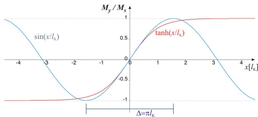
Figure 1: The red line displays the profile of an idealized one-dimensional 180^\circ domain wall in an infinitely extended ferromagnet with uniaxial anisotropy. The direction of the easy axis is along y and the red line displays the y -component of the normalized magnetization. In the case of a Bloch wall, the x component is zero for all x . The corresponding domain wall width \Delta = \pi l_K according to Lilley is sketched below. Close to the middle of the domain wall, x = 0 , the domain wall profile is very similar to that of a spin spiral with wave length 2\pi l_K = 2\Delta , displayed in blue.
