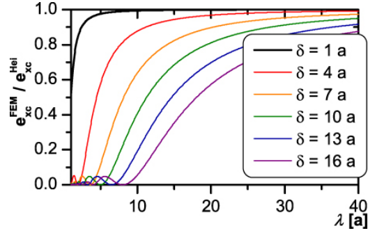
Figure 8: The graph shows the numerical value e_{xc}^{FEM}(\lambda, \delta) in units of the exchange energy calculated with the Heisenberg model as a function of \lambda . The behavior is very similar to that shown in Fig. 5. This shows that, for all practical cases, the discretization error dominates largely over the errors resulting from the use of eq. (7). In spite of their systematically opposite tendency, the two types of errors do not cancel each other. The material is BCC n.n. [35].
