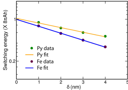
Figure 3: The energy required to switch a vortex core is equal to the energy needed to generate a Bloch point. According to analytic theory, the value of this energy is 8\pi Ah (see text). Numerical simulations systematically underestimate this switching energy, even if the cell size \delta is well below the exchange length l_K . However, an extrapolation to zero cell size reconciles the results, yielding perfect agreement with analytic theory. This is confirmed for different magnetic materials (from Ref.[27]).
