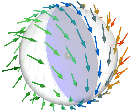
Figure 2: The image displays an example of the micromagnetic structure in the vicinity of a Bloch point. Such point singularities in the three-dimensional vector field \mathbf{M}(\mathbf{r}, t) generate highly frustrated and strongly inhomogeneous regions. In the center of the Bloch point, no direction of the magnetization can be defined. Each subset of the magnetization field defined on the surface of a small sphere containing the Bloch point fills the entire directional space, i.e. , it contains at least one magnetization vector pointing in any chosen direction.
