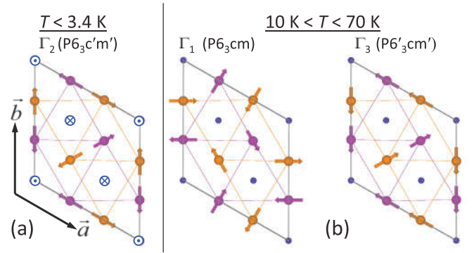
FIG. 2. (Color online) (a) Magnetic structure in the low-temperature ferrimagnetic phase, present below T_N^{\text{Dy}} = 3.4 K. The structure belongs to the P6_3c'm' magnetic space group ( \Gamma_2 irreducible representation). Mn ions at z = 0 are shown in purple, Mn ions at z = 1/2 are shown in orange, and the rare-earth ions are shown in blue. The refined ordered moments are 3.7 \pm 0.4 \mu_B on the Mn ions and 3.1 \pm 0.3 \mu_B on the Dy ions. (b) The two possible magnetic structures for the antiferromagnetic phase: P6_3cm magnetic space group ( \Gamma_1 irreducible representation) on the left and P6_3c'm' magnetic space group ( \Gamma_3 ) on the right. The Mn ordered moment is 3.5 \pm 0.4 \mu_B . Any Dy ordered moment in this temperature range is too small to be measured by neutron diffraction. The structural unit cell is outlined in gray.
