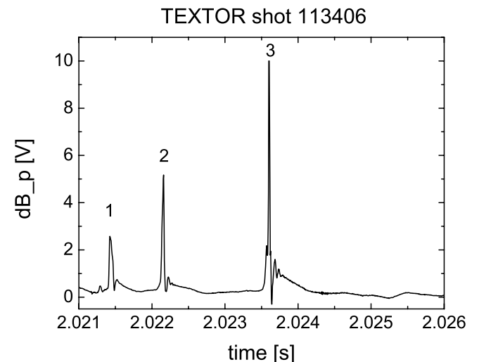
FIG. 4. Poloidal magnetic oscillations measured by a Mirnov coil on the LFS and corresponding to the 3 RE bursts in Fig. 2(a).
