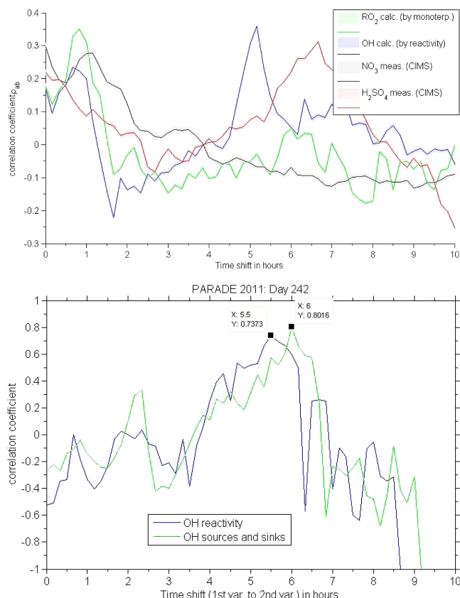
Figure 13. Top: cross-correlation of particle formation at 5 nm with \text{RO}_2(\text{terp.}) , OH, \text{NO}_3 and \text{H}_2\text{SO}_4 . Bottom: cross-correlation between the particle formation rate at 5 nm and the estimated OH concentration using two different approaches. The maximum is found at \tau of 5.5 h (6 h for the budget approach), resulting in a GR of 3.5 \text{ nm}/5.5 \text{ h} = 0.6 \text{ nm h}^{-1} .
