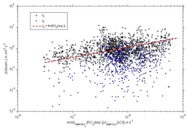
Figure 16. Scatter plot of the activation term in Eq. (5) vs. the formation rates at 3 and 5 nm.
