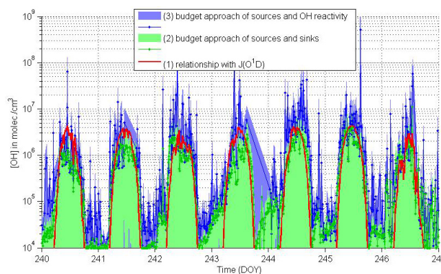
Figure 4. Concentrations of ambient OH calculated through different approaches for a period during PARADE (DOY 240–247): (1) J(\text{O}^1\text{D}) -based formulation, (2) budget approach of measured individual sources and sinks as well as (3) budget approach of measured individual sources and OH reactivity. The extended version can be found in the Supplement (Sect. B, Fig. S6, p. 10).
