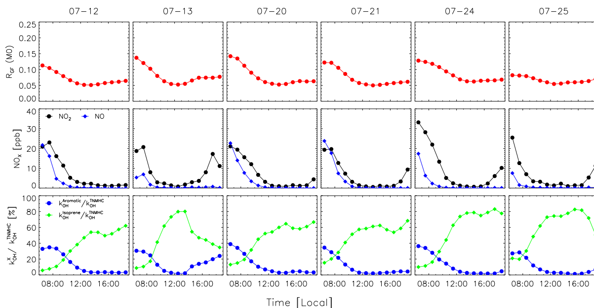
Figure 5. Time series of modeled R_{GF} (by the model base case), measured NO and NO 2 concentrations and NMHC compositions for the 6 cloud-free days during the PRIDE-PRD2006 campaign. The NMHC composition is expressed as the fraction of OH reactivity of a certain type of NMHC to that of the total NMHC.
