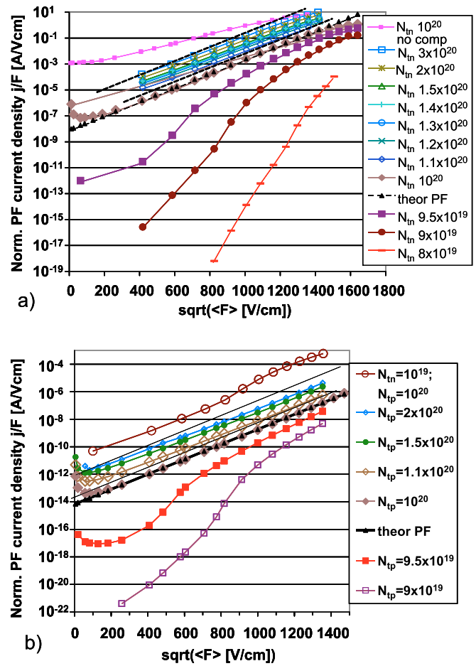
FIG. 10. Comparison of simulation data (PF-plot) with implementation of PFE for nearly compensated traps at constant parameters (see text) except: (a) the density of donor-like traps, N_{\text{tn}} , which was varied around the constant density of the acceptor-like traps, N_{\text{tp}} = 10^{20} \text{ cm}^{-3} from over-compensation, N_{\text{tn}} < N_{\text{tp}} (lower curves) to under-compensation, N_{\text{tn}} > N_{\text{tp}} (upper curves) for electron dominated current, and (b) the density of acceptor-like traps, N_{\text{tp}} , which was varied around the constant density of the donor-like traps, N_{\text{tn}} = 10^{20} \text{ cm}^{-3} from over-compensation, N_{\text{tp}} < N_{\text{tn}} (lower curves) to under-compensation, N_{\text{tp}} > N_{\text{tn}} (upper curves) for hole dominated current. In each figure, one curve with high under-compensation was added for comparison. The straight lines for selected curves correspond to the expected PFE behavior normalized at high applied fields.
