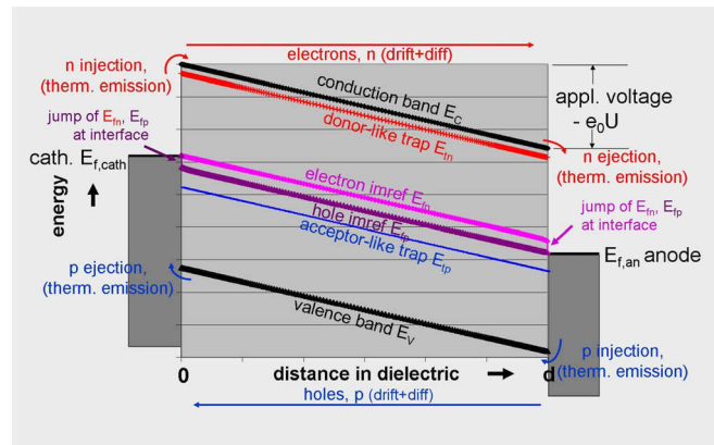
FIG. 3. Schematic sketch of a band diagram for the combined model used for simulation.
