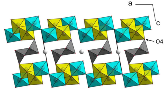
FIG. 8. (Color online) Crystal structure of \text{Li}_{0.33}\text{V}_2\text{O}_5 at 12.87 GPa ( \text{C2/m} , Z = 6 ). The polyhedra around the V1, V2, and V3 atoms are drawn yellow, cyan, and dark gray, respectively. The gray symbols are the Li atoms. The O4 oxygen atom is indicated.
