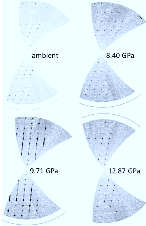
FIG. 7. Reconstructions of the reciprocal space in \beta - \text{Li}_{0.33}\text{V}_2\text{O}_5 at various pressures in the (h0l) projection. The reconstructions for the data below 9 GPa correspond to the ambient-pressure structure. The reconstruction for the data at 9.71 GPa corresponds to the intermediate phase in which strong one-dimensional diffuse scattering along c^* is observed. The reconstruction for the data at 12.87 GPa corresponds to the new polymorph whose crystal structure is discussed in this work. The angles \beta^* between a^* (a horizontal direction) and c^* at pressures below 9 GPa, at 9.71 GPa, and at 12.87 GPa are about 70^\circ , 85^\circ , and 80^\circ , respectively.
