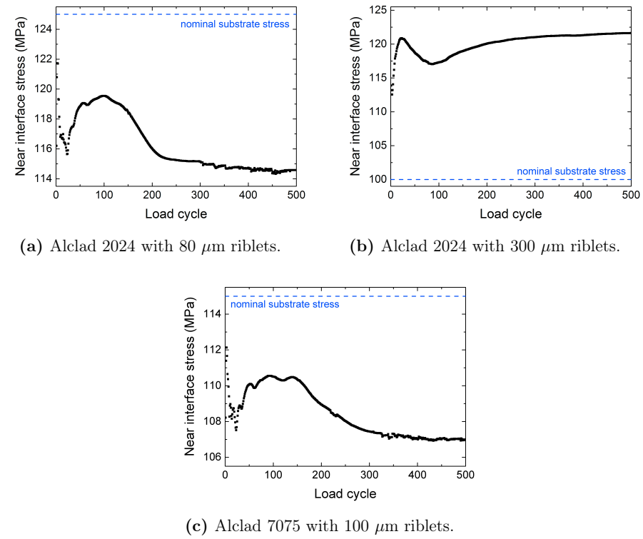
Figure 7.7: Saturation of stress redistribution in clad layer during cyclic loading.
