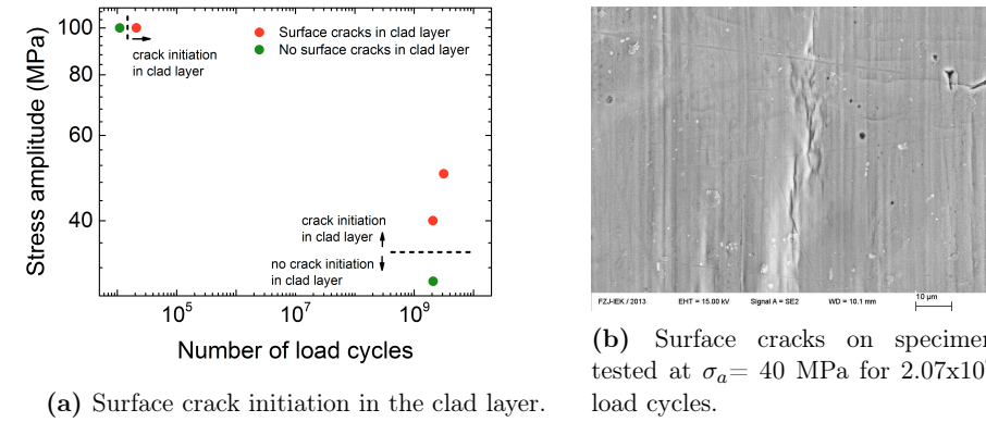
Figure 6.15: Initiation of surface cracks in Alclad 2024 material.
