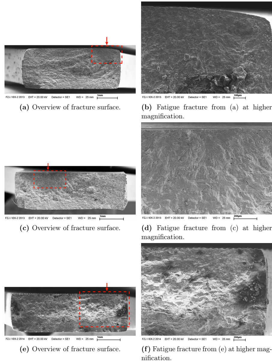
Figure 6.6: Fracture surfaces of bare flat AA 2024 specimens. (a) and (b) Flat specimen tested at \sigma_a = 135 MPa ( \sigma_{S.W.T.} = 116.2 MPa), N_f = 1.38 \times 10^9 . (c) and (d) Structured specimen with riblets normal to load direction tested at \sigma_a = 110 MPa, N_f = 2.07 \times 10^9 . (e) and (f) Structured specimen with riblets along load direction tested at \sigma_a = 140 MPa, N_f = 1.21 \times 10^8 .
