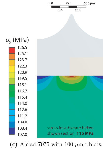
Figure 7.5: Effect of stress redistribution in the structured clad layer on substrate and interface stress during maximum load during the 500th load cycle.
