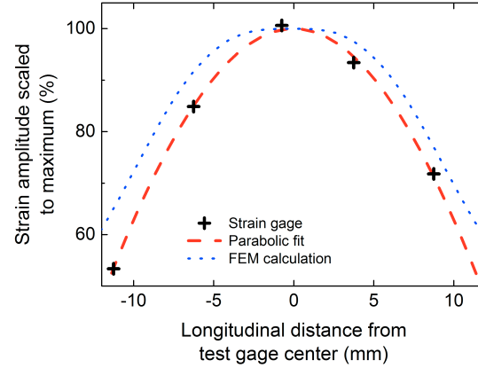
Figure 3.5: Strain distribution during ultrasonic fatigue testing.
