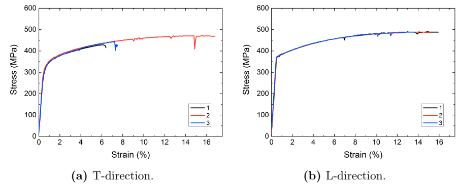
Figure 4.2: Tensile testing of 2 mm thick AA 2024 sheets.
