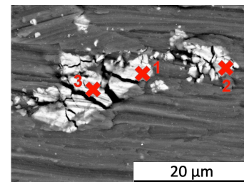
(b) Cracks at inclusions at higher magnification. The numbers indicate positions for EDX analysis.
