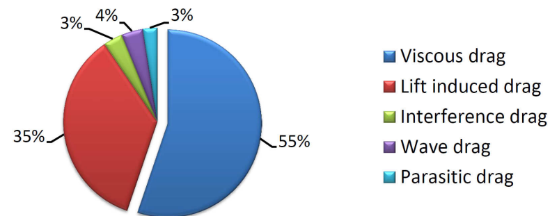
Figure 1.1: Drag breakdown of modern airplanes according to Schrauf et al. [1].
