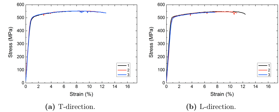
Figure 4.5: Tensile testing of 2 mm thick AA 7075 sheets.
