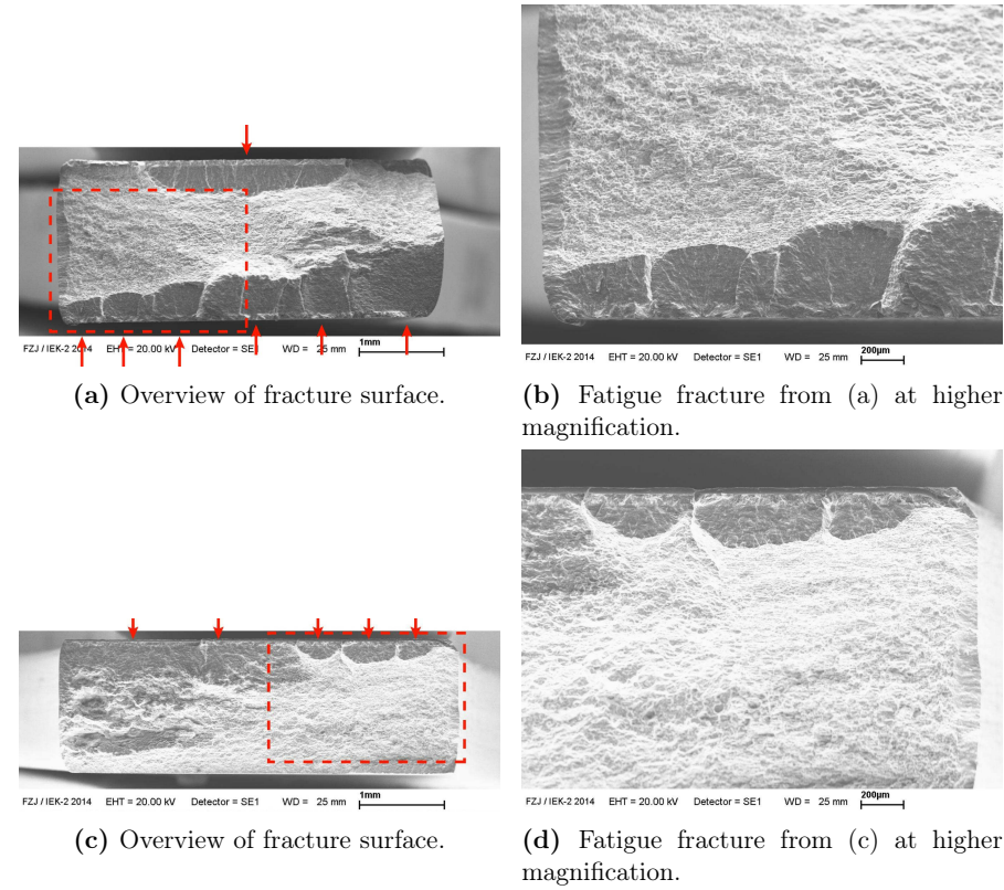
Figure 6.22: Fracture surfaces of Alclad 7075 specimens. (a) and (b) Flat specimen tested at \sigma_a = 120 MPa, N_f = 1.09 \times 10^6 . (c) and (d) Structured specimen with riblets normal to load direction tested at \sigma_a = 150 MPa, N_f = 5.55 \times 10^5 .
