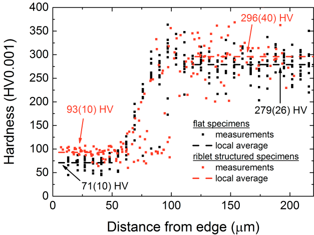
Figure 5.5: Micro indentation measurements of flat and riblet structured Alclad 7075.
