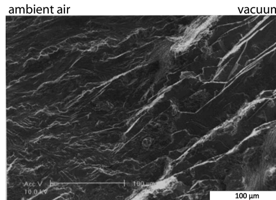
Figure 2.11: Influence of surrounding atmosphere on fracture surfaces of AA 7075 T6 at a cyclic stress intensity amplitude of 3.5 \text{ MPa}\sqrt{\text{m}} [15].
