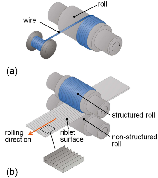
Figure 5.1: Rolling procedure for semicircular riblet geometry [134, 135]. (a) Preparation of the rolling equipment. (b) Rolling procedure.
