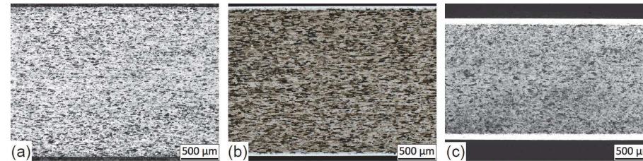
Figure 4.4: Polished cross sections of studied AA 2024 specimens. (a) 2 mm thick bare sheet. (b) 2 mm thick clad sheet. (c) 1.6 mm thick clad sheet.
