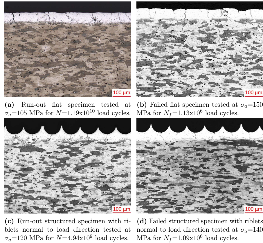
Figure 6.14: Polished cross sections of 2 mm thick Alclad 2024 material.
