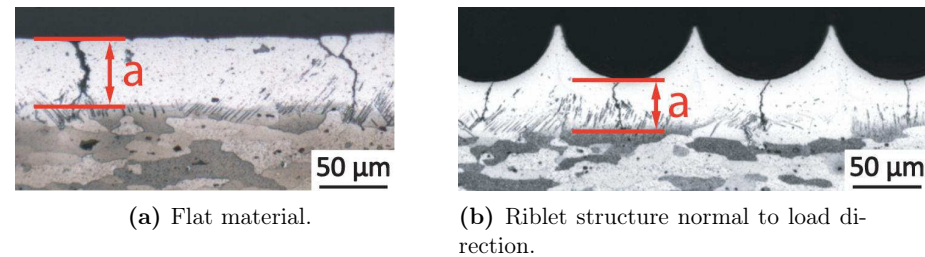
Figure 6.24: Definition of the crack length as equal to the local cladding thickness.
