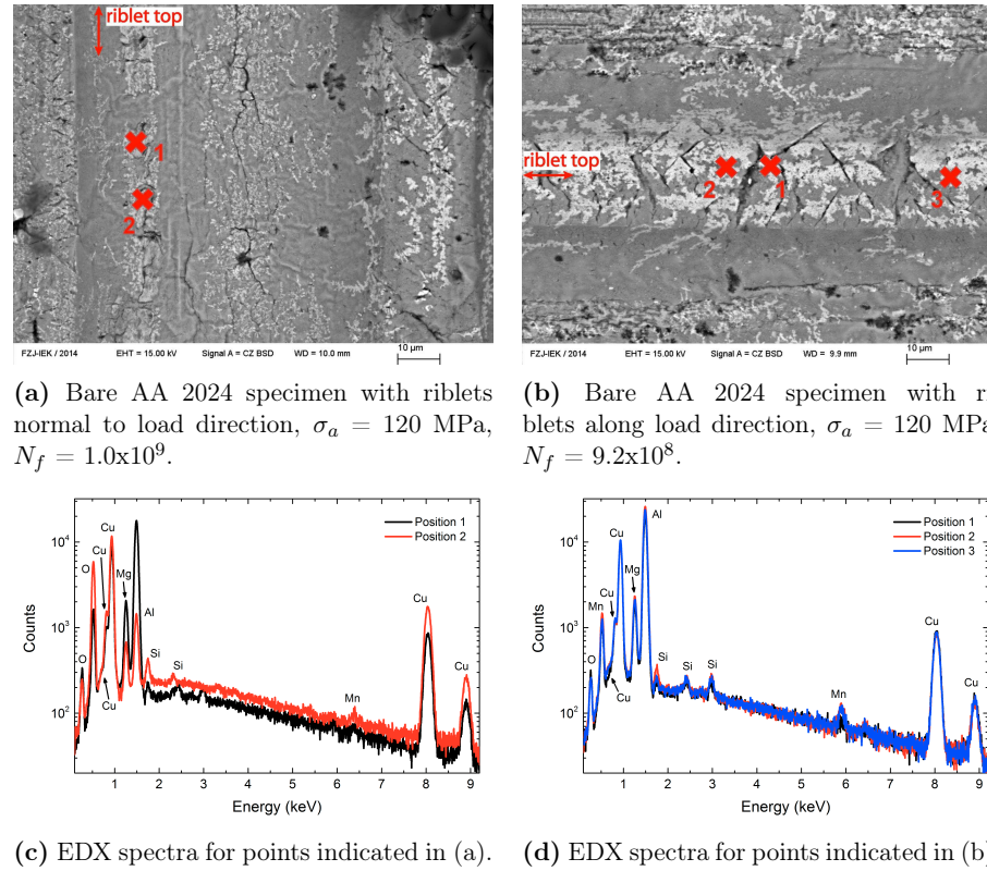
Figure 6.8: Surface cracks at riblet structured bare AA 2024 specimens with different riblet orientation.
