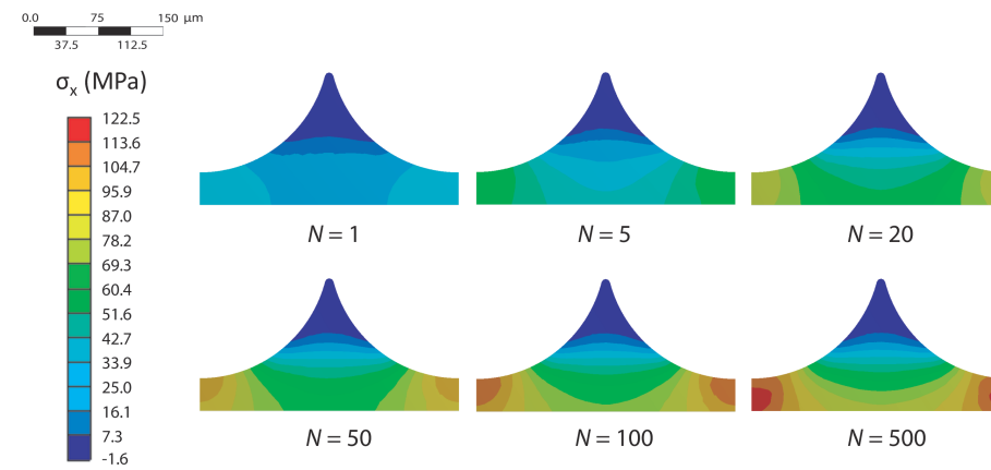
(b) 300 \mu\text{m} riblets in Alclad 2024.
