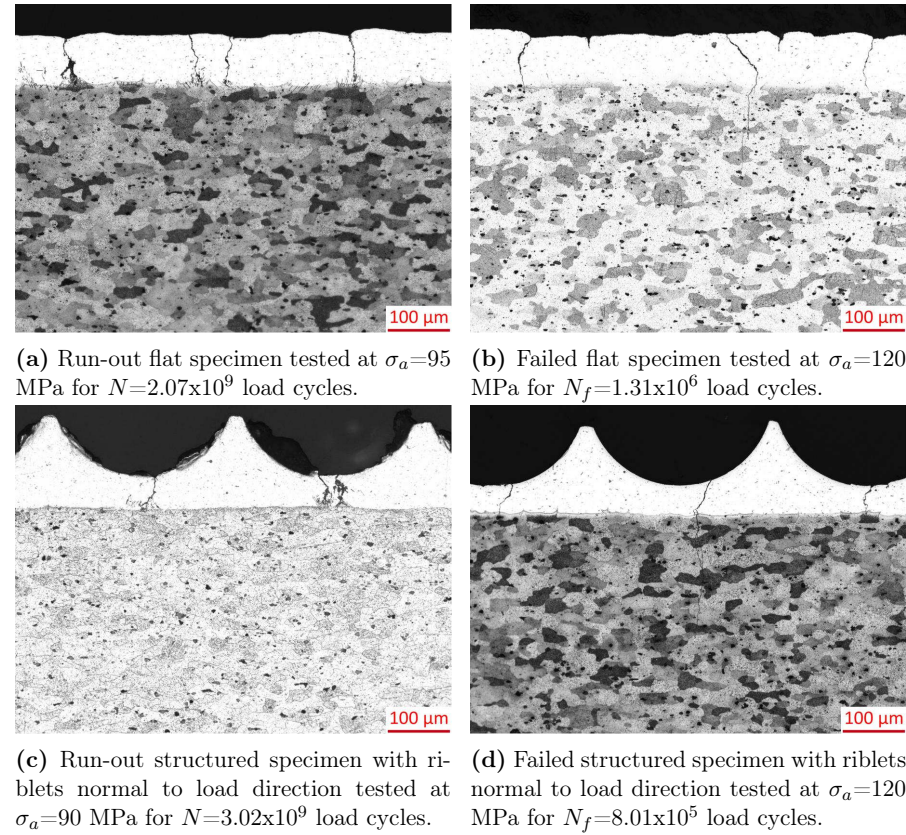
Figure 6.19: Polished cross sections of 1.6 mm thick Alclad 2024 material.
