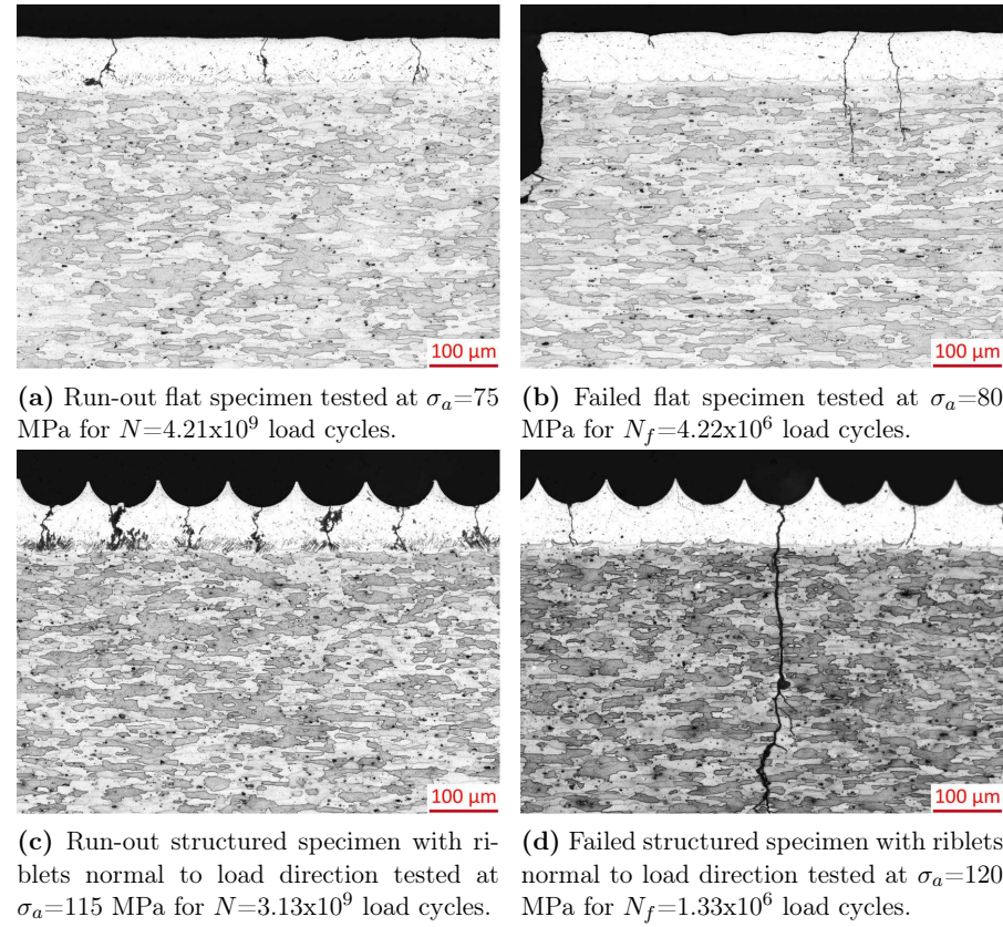
Figure 6.23: Polished cross sections of 2 mm thick Alclad 7075 material.
