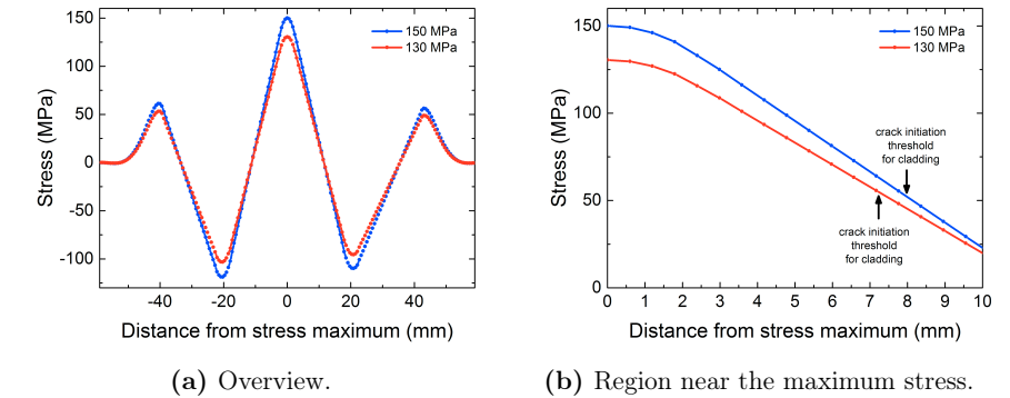
Figure 8.5: Longitudinal stress distribution at maximum load in bending testing.
