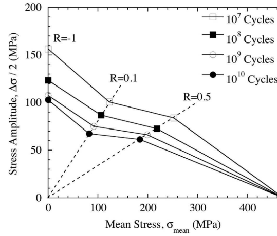
Figure 2.12: Haigh diagram from the study of Mayer et al. [14] for AA 2024 T351 illustrating the influence of mean stress on fatigue life.
