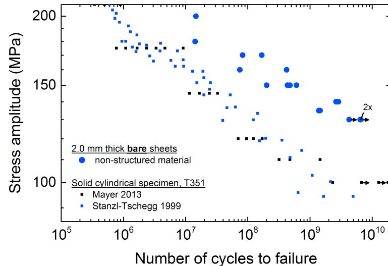
Figure 6.1: S/N -curve for flat AA 2024 bare sheets compared to literature data from Mayer [14] and Stanzl-Tschegg [11].
