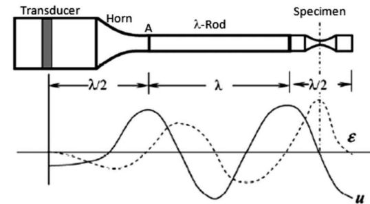
Figure 3.1: Principle of the ultrasonic fatigue testing equipment with distribution of displacement ( u ) and strain ( \epsilon ) [92].
