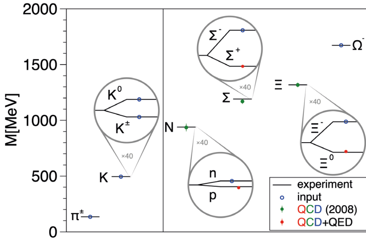
Figure 2: Mass splittings. Shown are individual masses from Figure 1, with the results [1] on the mass splittings shown in 40x magnification.
