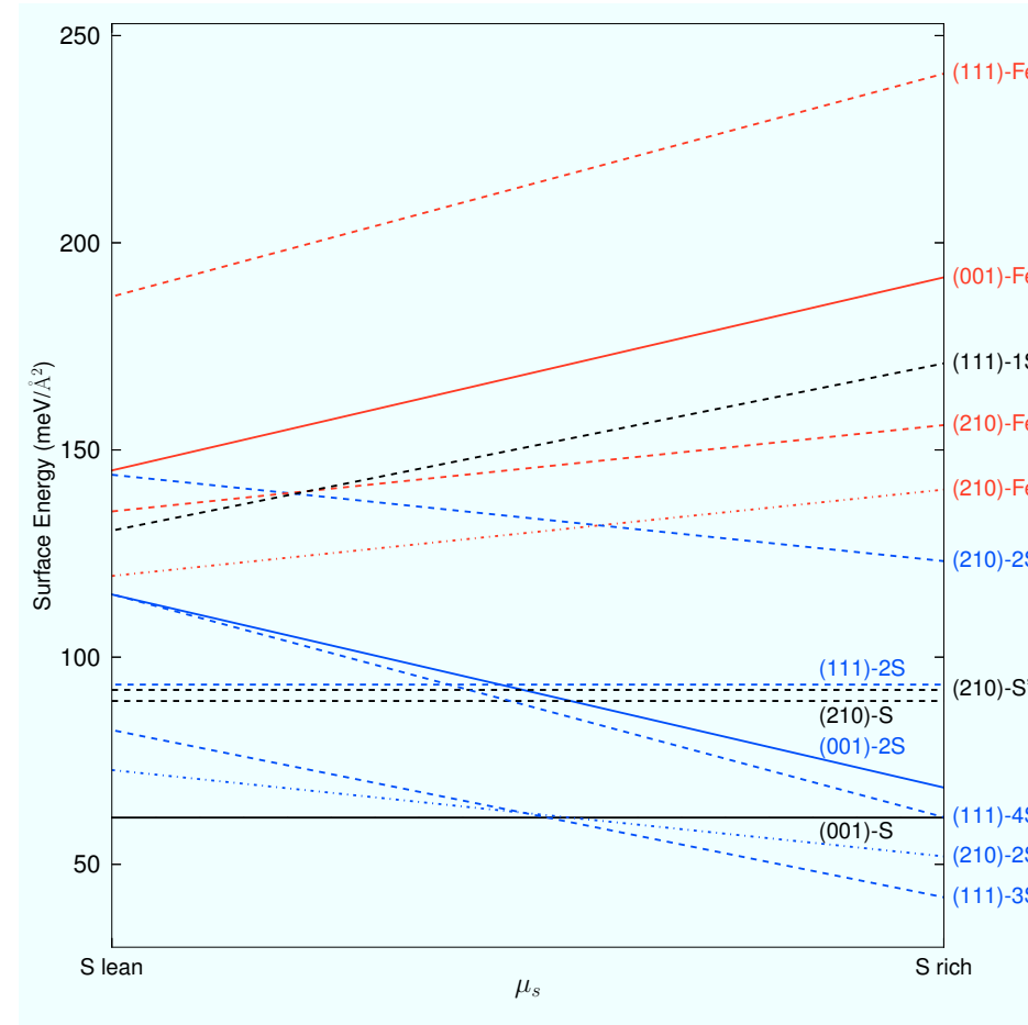
Figure 11.4.: The surface energies of the 14 investigated iron pyrite films of different terminations and orientations depending on the chemical potential of S, denoted as \mu_S . The color code is as follows: the Fe terminated films are red, the single S terminated films are black and the multiple S terminated films are blue. The surface energies of the films of (001) orientation are drawn in solid lines, whereas the (111) films and primed (210) films are indicated as dashed and the unprimed (210) films as dashed-dotted lines. The minimum and maximum of \mu_S , denoted as S lean and S rich limit, corresponds to the experimental situation where the conditions cause a formation of bcc-Fe or S_8 on the surface in a synthesis. The difference between the S lean and S rich limit is about 0.7 eV.
