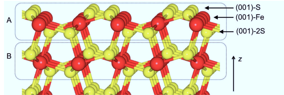
Figure 11.2.: The top-most 6 atomic layers of a (001)-S iron pyrite film from side view. The Fe atoms are indicated in red and the S atoms in yellow. The arrows indicate the three possible terminations for the (001) iron pyrite films, e.g. the (001)-Fe film has the Fe atomic layer as top-most layer and the (001)-2S film exhibits the two atomic layers of S on top. There are only three different terminations for the (001) orientation and not 6, because the S-Fe-S layers A and B are equivalent via symmetry.
