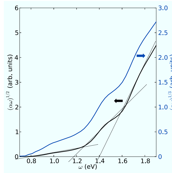
Figure 7.10.: The tail of the optical absorption of Fig. 7.9 in the range of 0.7 to 1.9 eV has been examined in case of an allowed indirect transition ( n = 1/2 , black curve) and in case of a forbidden indirect transition ( n = 1/3 , blue curve) for the optical band gap as it is presented in the reference [34]. The left y -axis corresponds to the black curve, whereas the right y -axis is valid for the blue curve. For the case of n = 1/2 linear fits are indicated for the three distinct regions of pronounced linear behavior by the thin, dashed black lines.
