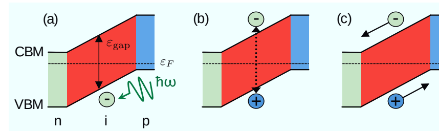
Figure 6.1.: The basic principle of a solar cell is based on the sequence of the following steps. The vertical direction in the figure can be interpreted as an energy axis and from left to right we show the different materials the solar cell is made: the p - and n -doped semiconducting layers and the undoped intrinsic (i) one. The location of the Fermi energy \epsilon_F is indicated by the dashed line. (a) A photon is absorbed in the intrinsic semiconducting layer. (b) An electron from the valence band (VBM - valence band maximum) is excited into the conduction bands (CBM - conduction band minimum). The remaining hole in the valence band is coupled to the electron. Both together form a so-called exciton. (c) An internal electric field caused by the space-charges in the p - and n -doped semiconducting layers separates the charge carriers.
