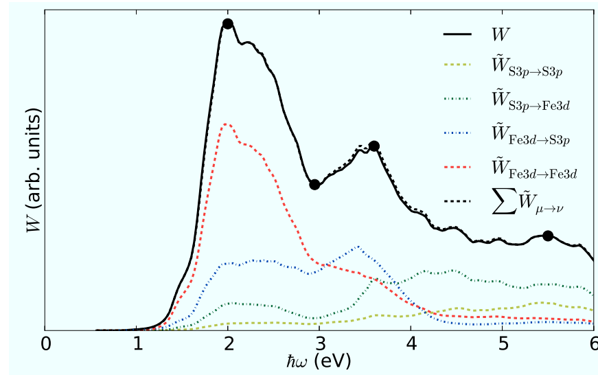
Figure B.2.: The total transition rate W of iron pyrite is presented as a black solid curve. The orbital-resolved transition rates W_{\mu \rightarrow \nu} do not add up to the total transition rate, and thus a system of linear equations is solved to find factors such that the multiplied transition rates \tilde{W}_{\mu \rightarrow \nu} approximately sum up to the total transition rate. The most important orbital-resolved transition rates are those of the Fe 3d -Fe 3d (red dashed curve), the Fe 3d -S 3p (blue dashed-dotted curve), the S 3p -Fe 3d (green dashed-dotted curve) and the S 3p -S 3p transitions (yellow dashed curve) within the energy range of 6 eV. The sum of these four transition rates is indicated as black dashed curve. The four large black markers show the chosen values for the total transition used in the system of linear equations to obtain reasonable multiplication factors for the orbital-resolved transition rates.
