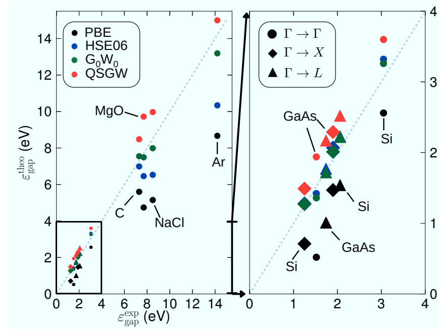
Figure A.1.: The transition energies of \Gamma \rightarrow \Gamma (circles) for Si, C, Ar, MgO, NaCl and GaAs, and additionally the transition energies of \Gamma \rightarrow X (diamonds) and \Gamma \rightarrow L (triangles) for Si and GaAs are displayed. The transition energies are calculated within GGA-PBE (black), HSE06 (blue), G_0W_0 @PBE (green) and QSGW (red), and they are plotted against the values measured in experiment. Hence, a value on the gray dashed linear curve means a perfect agreement between theory and experiment. Since the results within the energy scale between 0 and 4 eV are difficult to display in the left panel, a zoom into the corresponding energy range is shown in the right panel. The transition energies are also listed in table A.2.
