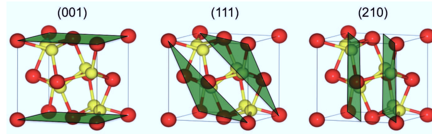
Figure 11.1.: The lattice planes of the crystallographic orientations (001), (111) and (210) in the bulk unit cell of iron pyrite.
