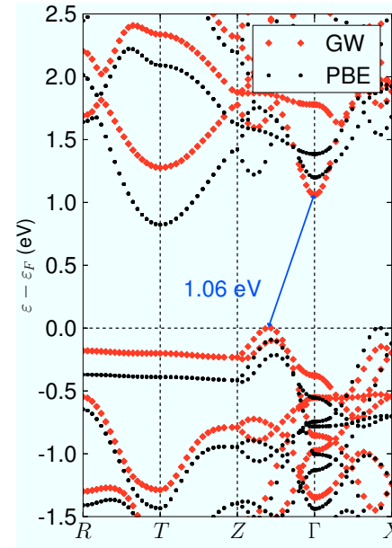
Figure 9.3.: The electronic band structure of iron marcasite using the structural parameters from experiment within GGA-PBE (black dots) and G_0W_0@PBE (red diamonds) is displayed. The blue arrow indicates the fundamental band gap predicted by the GW calculation.
