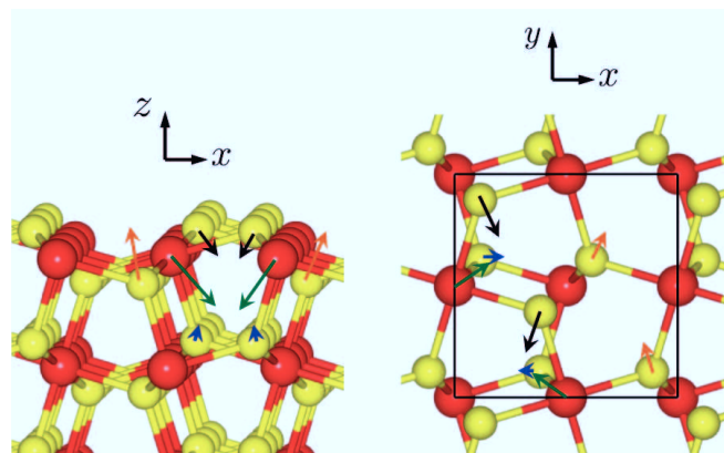
Figure 11.3.: The displacements of the atoms in the first four atomic layers of (001)-S within the structural relaxation are indicated in arrows using a side (left panel) and top view (right panel) of the structure. The arrows are not true to scale, but the relative size among them is approximately reproduced. The displacements are color coded depending on the atoms: S_{1a} and S_{1b} (black), Fe_{1a} and Fe_{1b} (green), S_{2a} and S_{2b} (orange) and S_{3a} and S_{3b} (blue). The quadratic 2-dimensional unit cell of the (001) film is depicted as black frame in the top view.
