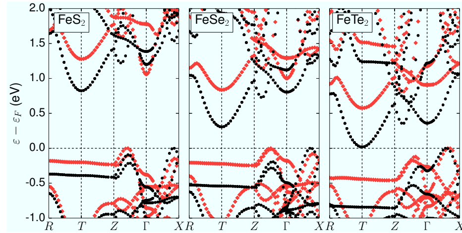
Figure 10.5.: The electronic band structure of \text{FeS}_2 (left), \text{FeSe}_2 (center) and \text{FeTe}_2 (right) using the structural parameters from table 10.1 within the G_0W_0@PBE (red diamonds) and “plain” GGA-PBE calculation (black dots). The sizes of the fundamental band gaps within GGA-PBE and GW are listed in table 10.3.
