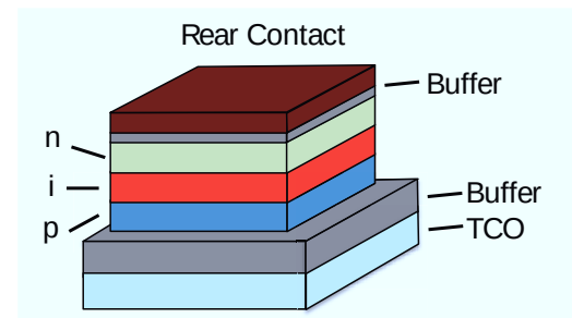
Figure 6.2.: A schematic figure of a typical p-i-n thin-film solar cell, consisting of the intrinsic absorber layer i sandwiched by a p - and n -doped semiconducting layer. The two buffer layers are usually needed to improve the growth conditions and to increase the performance of the solar cell. On the side where the light enters, a transparent conductive oxide (TCO) collects the charges, whereas a nontransparent metallic contact is used on the rear side.
