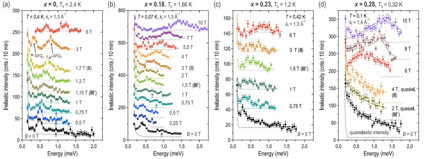
FIG. 2. (Color online) INS spectra measured at the AFQ wave vector, R(\frac{1}{2} \frac{1}{2} \frac{1}{2}) , in different magnetic fields \mathbf{B} \parallel (1\bar{1}0) for (a) x = 0 , (b) x = 0.18 , (c) x = 0.23 , (d) x = 0.28 . The spectra are shifted vertically for clarity, the dashed lines indicating the background baseline for each spectrum. Solid lines represent fits described in the text.
