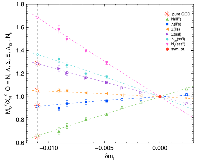
FIG. 5 (color online). The baryon fan plot for the \Sigma - and \Lambda -type particles \bar{M}_O^2 ( O = N, \Lambda, \Sigma, \Xi, \Lambda_{2s}, N_s ) versus \delta m_l . Filled up triangles, squares, left triangles, right triangles, diamonds and down triangles are the N(l'l'') , \Lambda(l'l's) , \Sigma(l's) , \Xi(ssl) , \Lambda_{2s}(ss'l) and N_s(sss'') results respectively using 32^3 \times 64 sized lattices. The common symmetric point is the filled circle. The open up triangles, left triangles, right triangles and down triangles are from comparison 24^3 \times 48 sized lattices (and not used in the fits here). The vertical dashed line from Eq. (79) is the n_f = 2 + 1 pure QCD physical point, with the open circles being the numerically determined pure QCD hadron mass ratios for 2 + 1 quark flavors. For comparison, the stars represent the average of the (\text{mass})^2 of M_N^{*2}(l'l'') = (M_n^{\text{exp}2}(ddu) + M_p^{\text{exp}2}(uud))/2 , M_\Lambda^{*2}(l's) = M_{\Lambda^0}^{\text{exp}2}(uds) , M_\Sigma^{*2}(l's) = (M_{\Sigma^-}^{\text{exp}2}(dds) + M_{\Sigma^+}^{\text{exp}2}(uus))/2 and M_\Xi^{*2}(ssl) = (M_{\Xi^-}^{\text{exp}2}(ssd) + M_{\Xi^0}^{\text{exp}2}(ssu))/2 .
