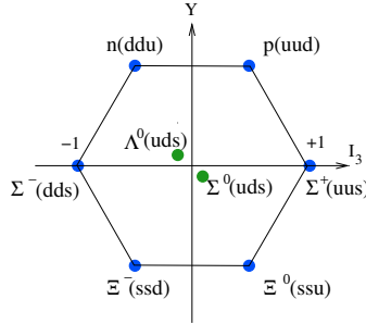
Figure 1: The baryon octet in the I_3 - Y plane.
