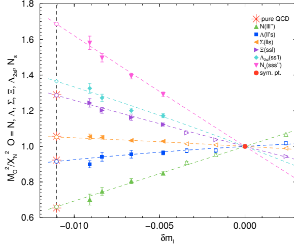
Figure 4: The baryon ‘fan’ plot for the ‘ N ’ and ‘ \Lambda ’ type particles \tilde{M}_{N_O}^2 ( N_O = N, \Sigma, \Xi, N_s ) and \tilde{M}_{\Lambda_O}^2 ( \Lambda_O = N, \Lambda, \Lambda_{12s}, N_s ) versus \delta m_l . The symbols are all unitary data. (The opaque triangular symbols are from comparison 24^3 \times 48 sized lattices and not used in the fits here.) The common symmetric point is the filled circle. The vertical dashed line is the N_f = 2 + 1 pure QCD physical point, with the opaque circles being the numerically determined pure QCD hadron mass ratios for 2 + 1 quark flavours. For comparison, the stars represent the average of the (\text{mass})^2 of M_N^{*2}(III'') = (M_n^{\text{exp}2}(ddu) + M_p^{\text{exp}2}(uud))/2 , M_{\Lambda}^{*2}(II's) = M_{\Lambda^0}^{\text{exp}2}(uds) , M_{\Sigma}^{*2}(II's) = (M_{\Sigma^-}^{\text{exp}2}(dds) + M_{\Sigma^+}^{\text{exp}2}(uus))/2 and M_{\Xi}^{*2}(ssl) = (M_{\Xi^-}^{\text{exp}2}(ssd) + M_{\Xi^0}^{\text{exp}2}(ssu))/2 .
