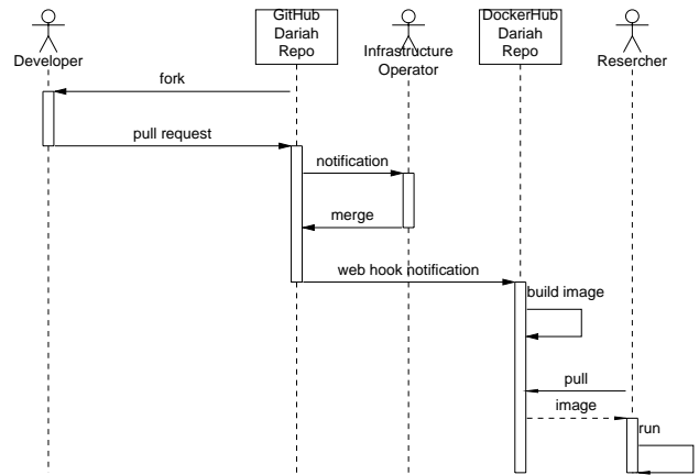
Figure 1. Proposed software sharing life cycle
