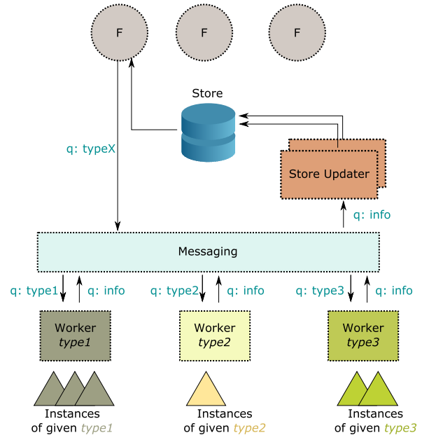
Figure 2. Architecture of the dynamic Software-as-a-Service
