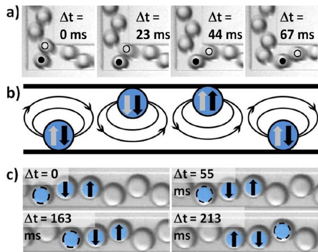
Fig. 6 a) Microscopy time series showing the droplet reorganisation at a 90° bend. b) Sketch indicating the relevant hydrodynamic interactions between the droplets in the co-moving frame. The transverse forces resulting from leading and trailing droplets in a zigzag configuration with one ‘mismatch’ are shown as grey and black arrows, respectively. c) Time series of a transverse droplet motion for a single ‘mismatch’ as described in b); three drops are marked and the net transverse forces, i.e., the sum of the grey and black arrows in b), are shown as black arrows.
