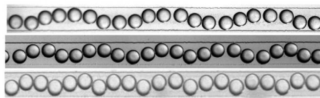
Fig. 7 Experimentally observed travelling sine waves as generated by periodic ‘mismatches’ using the setup shown in figure 6 having different droplet size ( R \approx 64 \mu\text{m} , R \approx 67 \mu\text{m} , and R \approx 70 \mu\text{m} from top to bottom) and different wavelength ( \lambda = 8a , \lambda = 6a , and \lambda = 4a from top to bottom).
