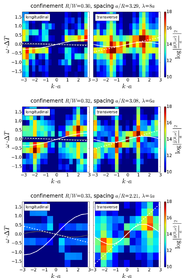
Fig. 8 Longitudinal and transverse power spectra of the droplet oscillations as calculated from experimental trajectories extracted from microscopy time series corresponding to the waves shown in Fig. 7.
