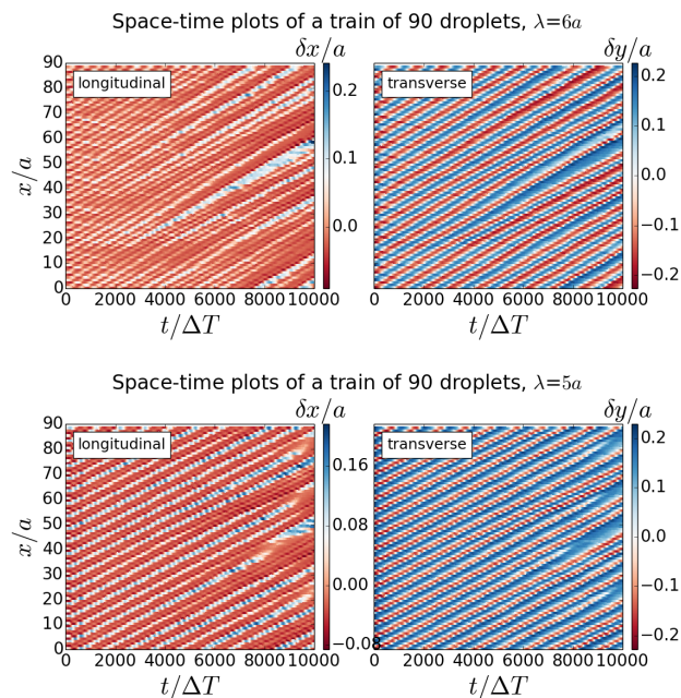
Fig. 12 Space-time plots of simulation runs of a train of 90 droplets forming a sine-like wave for wavelengths \lambda = 6a and \lambda = 5a .
