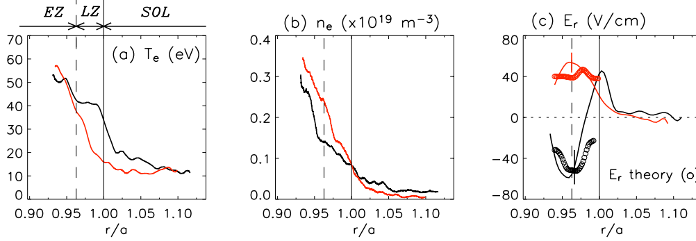
Fig. 1 Radial profiles of (a) electron temperature; (b) plasma density and (c) radial electric field before (black solid curves, w/o RMP) and during (red solid curves, with RMP) the static 6/2 DED measured by fast reciprocating probes at TEXTOR (# 99626). The radial locations are normalized by a . The vertical dashed line roughly separates the ergodic zone (EZ, left side) and the laminar zone (LZ, right side). The open circles in (c) show the simulated E_r .
