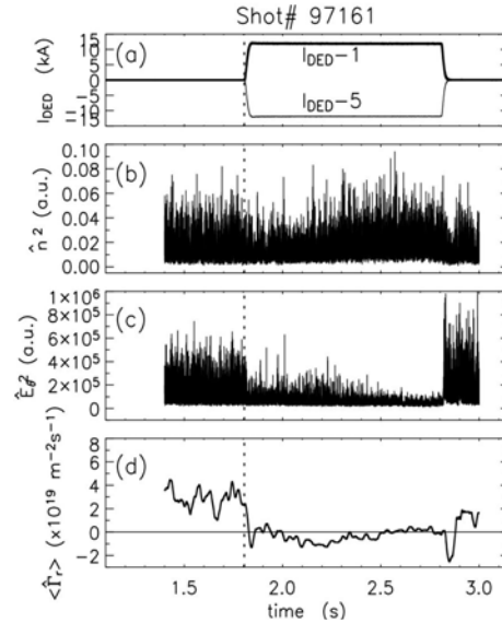
Fig. 2 Time traces of (a) DED currents; (b) power of density fluctuations; (c) power of poloidal electric field fluctuations and (d) ensemble-average of turbulent flux measured by a stationary probe in the ergodic region in static 12/4 DED. The vertical dotted lines denote the start time of the DED.
