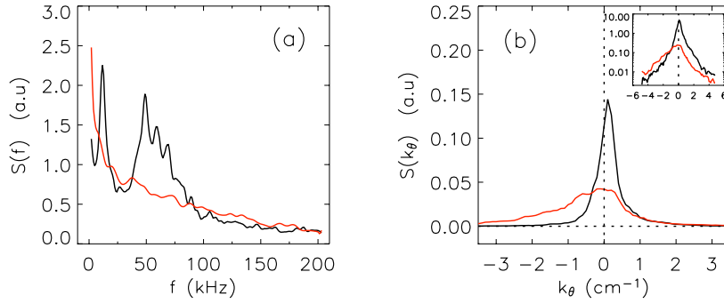
Fig. 3 Linear plot of (a) the frequency spectrum S(f) of density fluctuations and (b) the poloidal wave-number spectrum S(k_\theta) of potential fluctuations measured in the ergodic region ( \rho \approx 0.93 ) before (black curves) and during (red curves) the static m/n=6/2 DED. The magnitudes of S(k_\theta) are normalized by the total power before and during the DED, respectively. The semi-log plot in the inset of (b) displays their relative power. The k_\theta > 0 ( < 0 ) is in the electron (ion) diamagnetic drift direction.
