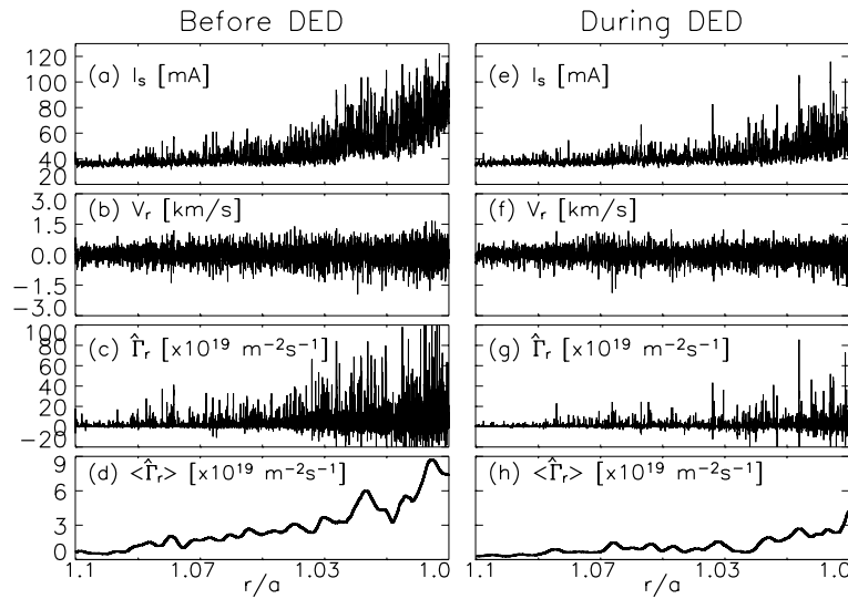
Fig. 4 Comparison of the I_s , V_r and \tilde{\Gamma}_r signals (versus normalized radial position) measured in the SOL before (left column) and during (right column) the static 6/2 DED (# 101795). Plotted in (d) and (h) are the ensemble-averaged turbulent flux. Corresponding parameters in the two columns are drawn in the same scale.
