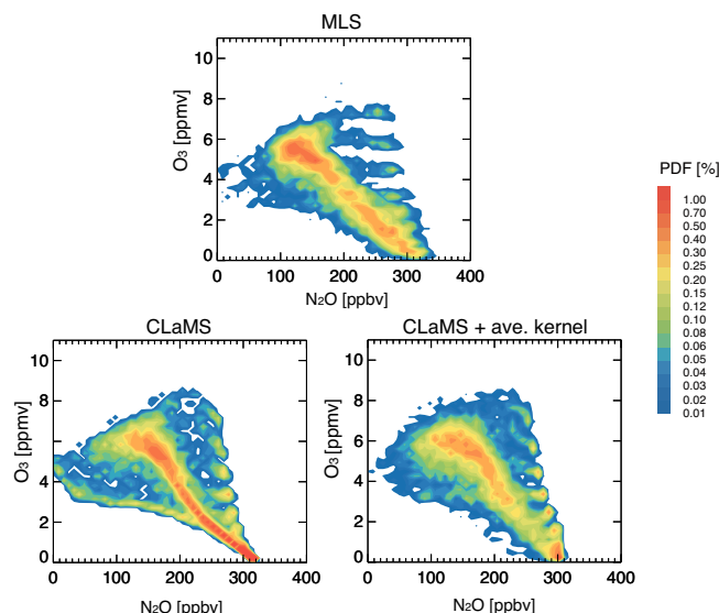
Figure A1. PDFs of \text{N}_2\text{O} – \text{O}_3 correlations on 15 February 2009 from MLS observations (top); from the reference CLaMS simulation without applying the averaging kernel (bottom left) and after applying the averaging kernel (bottom right).
