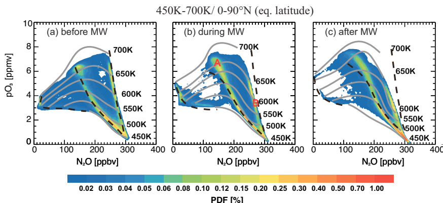
Figure 11. Impact of \text{O}_3 -chemistry on the temporal evolution of the \text{N}_2\text{O} - \text{O}_3 correlations. The PDFs are calculated from the \text{N}_2\text{O} - p\text{O}_3 correlations of APs with eq. latitudes 0 – 90^\circ N and potential temperatures 450 – 700 K. The considered time periods are the same as in Fig. 9. The dashed black curves fit the maxima of the \text{N}_2\text{O} - \text{O}_3 correlations (PDFs) derived from a CLaMS run with a full stratospheric ozone chemistry. The correlation for passive ozone ( p\text{O}_3 ) marked as A ( \text{N}_2\text{O} near 140 ppbv and p\text{O}_3 near 7400 ppbv) and the correlation marked as B ( \text{N}_2\text{O} near 140 ppbv and p\text{O}_3 near 7400 ppbv) show clear differences from the dashed curves showing simulation with full chemistry. The two groups of APs marked by those correlation features have been investigated in more detail of their ozone chemistry (see text).
