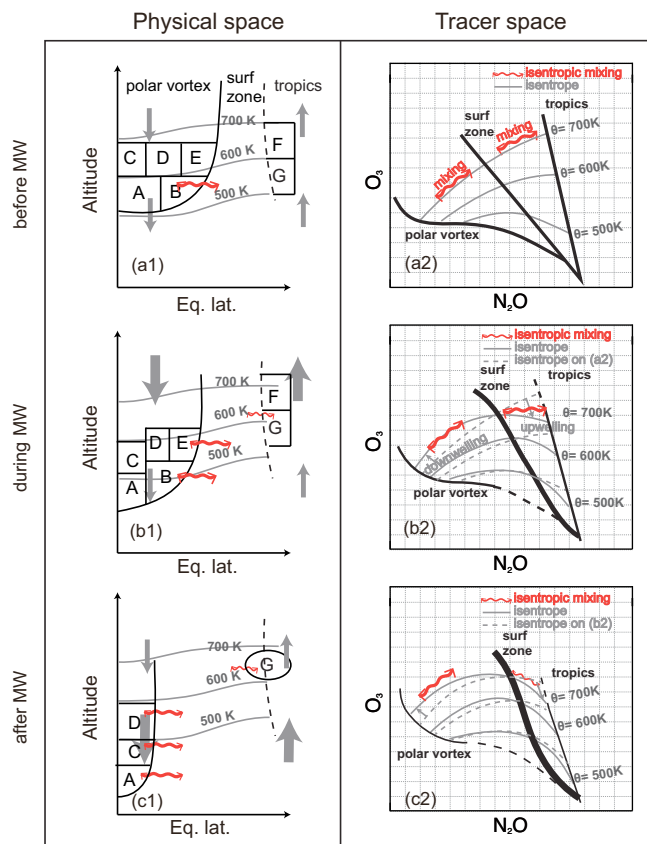
Figure 8. Schematic diagram of transport processes shown in physical space (left column) and tracer space ( \text{N}_2\text{O} – \text{O}_3 , right column) before (top), during (middle) and after (bottom) the major SSW. In the physical space (left column), equivalent latitudes are used as the horizontal coordinates to illustrate isentropic mixing (curved red arrows) and cross-isentropic transport (grey vertical arrows). The thickness of the grey arrows indicates the intensity of vertical motion. The characters denote exemplarily the vortex and tropical air masses which interact with the mid-latitude air. Black curves in (a2)–(c2) show respective \text{N}_2\text{O} – \text{O}_3 correlations. Grey lines denote the isentropic levels. In the tracer space, the position of isentropes before (dashed) and after (solid) the major SSW is also marked. The change of the position of a prescribed point in the tracer space along the isentropes quantifies isentropic mixing, whereas motion relative to these isentropes describes the effect of an idealized (mixing-free) cross-isentropic motion (up- or downwelling). Changes of the relative thickness of the different correlation branches mean their enhanced or weakened relative contributions to the composition of the considered part of the atmosphere (dashed lines indicate a possible missing part).
