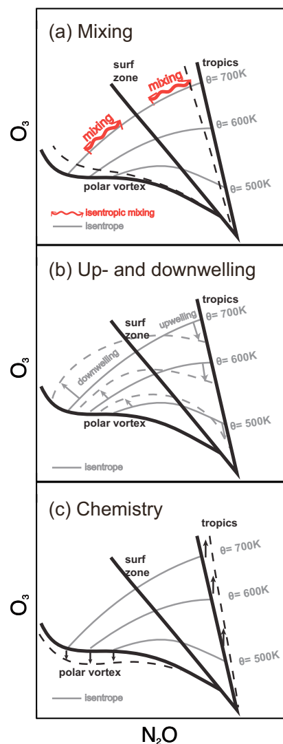
Figure 1. Schematic diagram showing the influences of (a) mixing, (b) up- and downwelling and (c) chemistry on \text{N}_2\text{O} – \text{O}_3 correlations.
