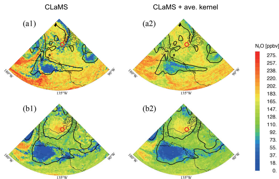
Figure A2. Spatial distribution of \text{N}_2\text{O} on 20 February 2009, i.e. almost 1 month after the major SSW at \theta = 550\text{ K} (top row) and 650\text{ K} (bottom row). Here the results of the reference run without and with the averaging kernel are shown in the left and right column, respectively. The black line denotes the vortex edge, the red circles are the noon-footprints calculated by the observed ACE profile through back and forward trajectory.
