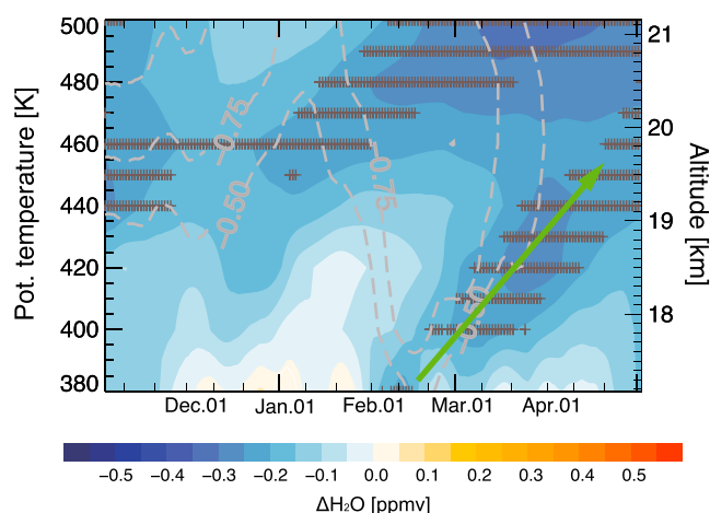
Figure 4. Differences of tropical ( 10^{\circ}\text{S} – 10^{\circ}\text{N} ) water vapor (colored) and temperature (gray contours) deseasonalized anomalies derived from the 35 year CLaMS simulation between winters in the 2000s and winters in the 1990s (2000s minus 1990s). Gray crosses indicate statistical confidence larger than 0.9 as derived from the Monte Carlo test.
