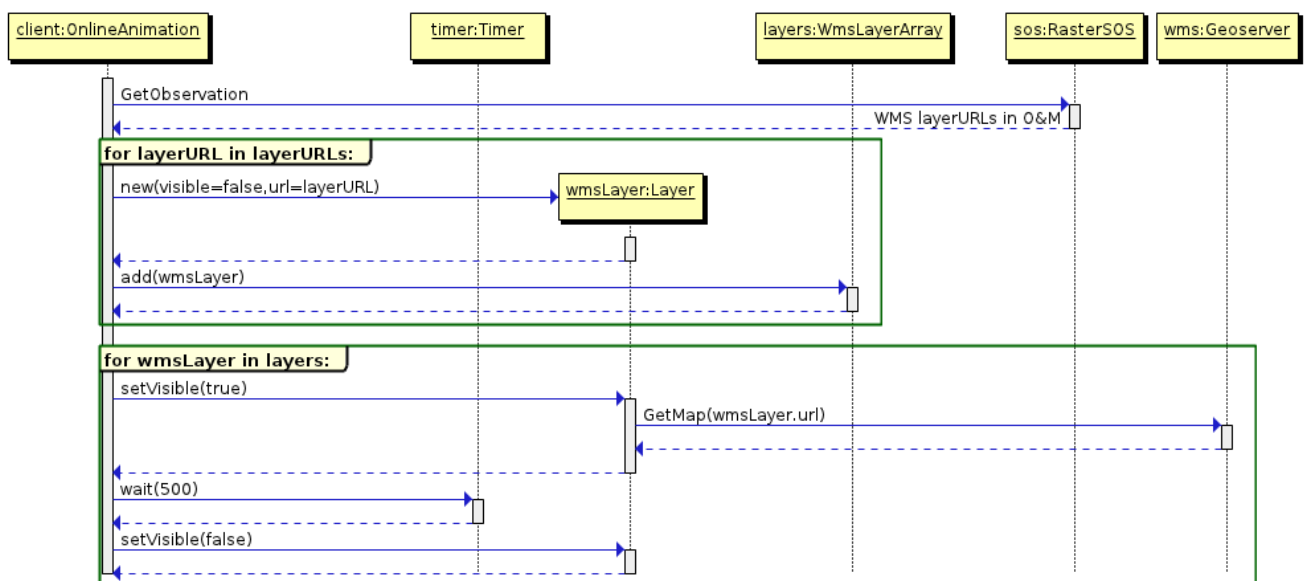
Figure 10. UML diagram of the communication between client, SOS, and WMS.
