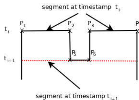
Figure 4. Sweep algorithm to scan orthogonal polygons.
