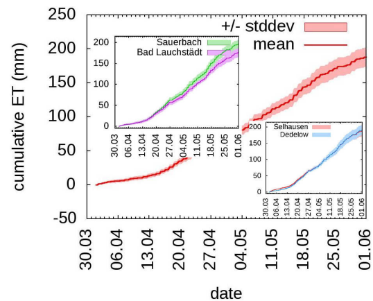
Figure 12. Cumulative evapotranspiration (mean \pm standard deviation) for the 12 crop lysimeters of the Bad Lauchstädt test site. The small picture shows the results separated in soil type groups.
