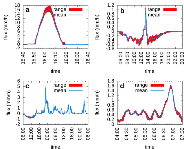
Figure 7. Short time dynamics of precipitation events for selected rain events of 9 May 2013 (a), 4 May 2013 (b), 26–28 April 2013 (c) and 12 April 2013 (d).
