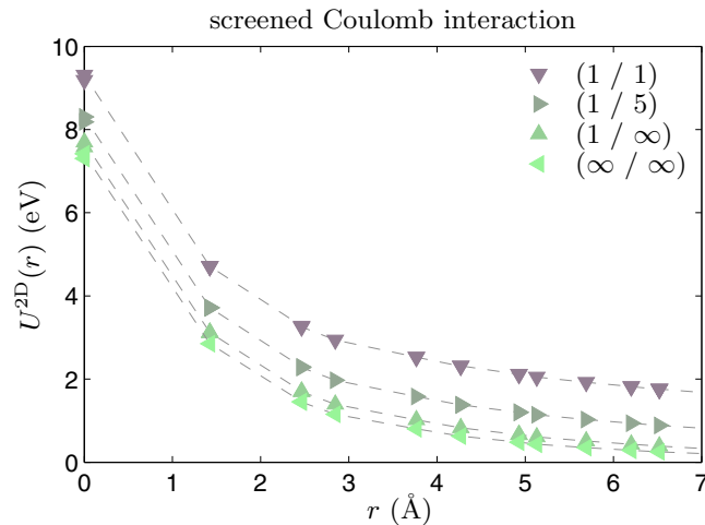
FIG. 7. (Color online) (left) WFCE density-density matrix elements of the background screened Coulomb interactions for bilayer graphene in real space for different dielectric surroundings ( \varepsilon_2/\varepsilon_3 ). (right) Corresponding dielectric functions in momentum space.
