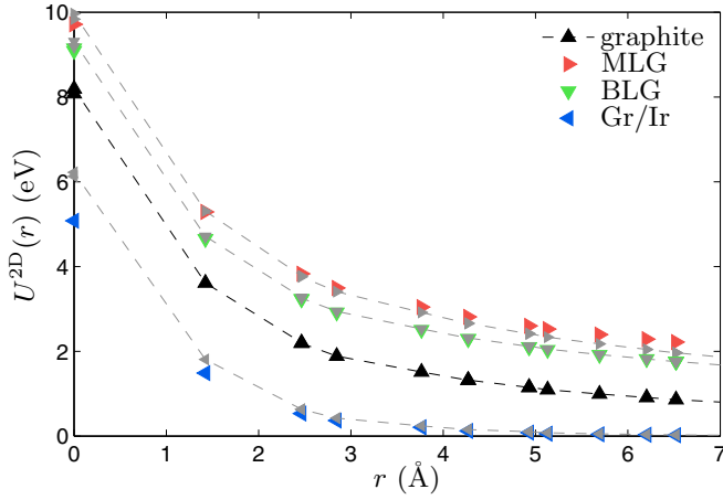
FIG. 6. (Color online) Density-density matrix elements of the screened Coulomb interactions for graphite, monolayer and bilayer graphene, and Gr/Ir in real space. Colored markers show ab initio values, and gray markers connected by dashed lines show the WFCE values.
