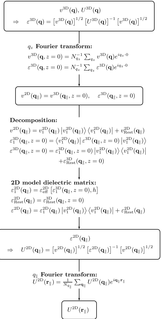
FIG. 2. Flowchart of the Wannier function continuum electrostatics (WFCE) algorithm to obtain the screened Coulomb matrix elements of a freestanding monolayer directly from the Coulomb interaction of the corresponding layered bulk material.
