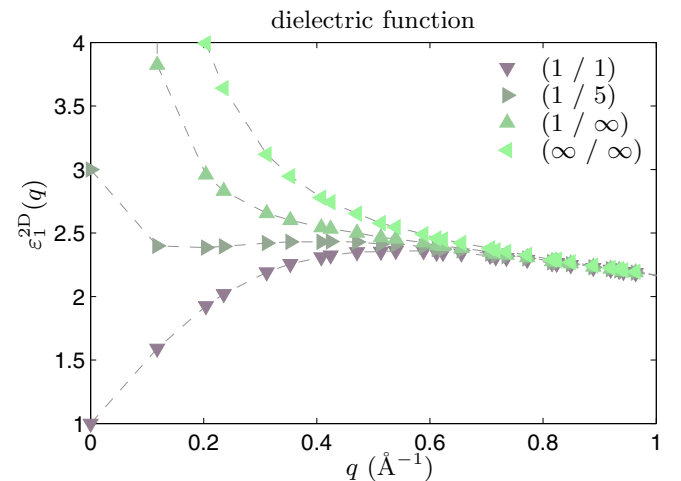
FIG. 7. (Color online) (left) WFCE density-density matrix elements of the background screened Coulomb interactions for bilayer graphene in real space for different dielectric surroundings ( \varepsilon_2/\varepsilon_3 ). (right) Corresponding dielectric functions in momentum space.
