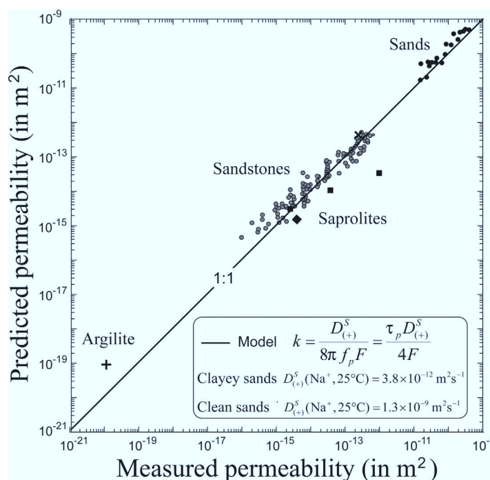
Figure 7. Comparison of permeability ( k ) modeled from SIP measurements of an electrical time constant ( \tau_p ) or relaxation frequency ( f_p ) and measured permeability (modified from Revil [2013]). Here D_{(+)}^S is the diffusion coefficient of cations in the Stern layer of the electrical double layer, and F is the formation factor.
