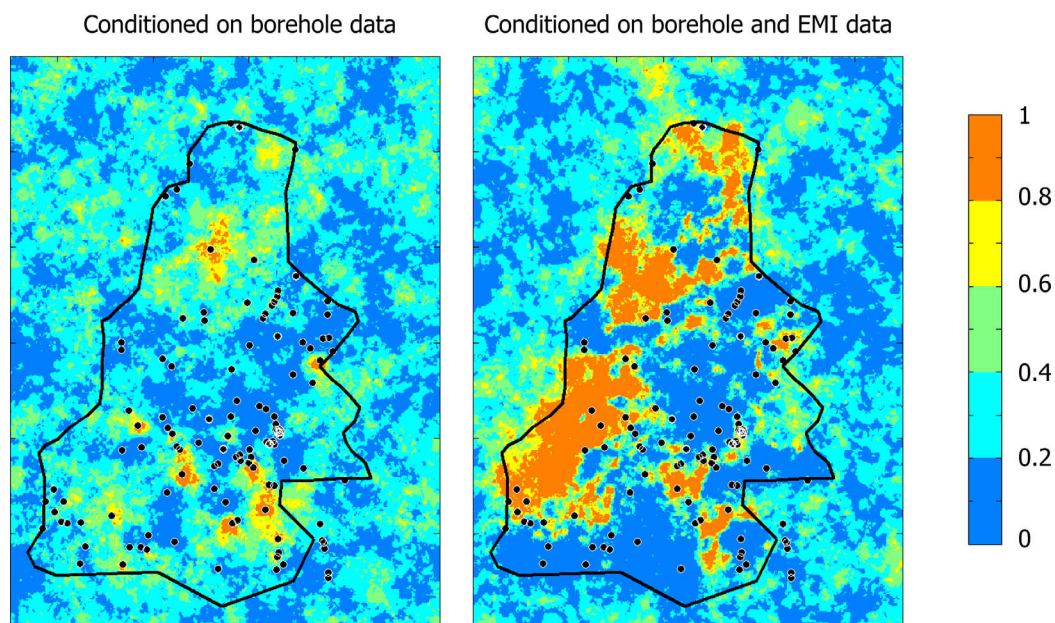
Figure 9. Simulated probabilities of sand fraction at a specific depth based on transitional probabilities conditioned on different data (modified after He et al. [2014]). (left) Probabilities conditioned on borehole data (locations shown as dots in the image). (right) Probabilities conditioned on borehole data and electrical conductivity obtained using airborne EMI. The black line shows the boundary of the geophysical survey. Each rectangular image represents an area of 108 km 2 . He et al. [2014] demonstrate the value of adding the geophysical data to this structural characterization problem.
