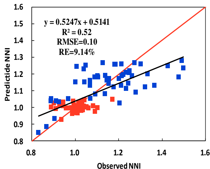
Figure 2. Relationship between observed and predicted NNI using MCARI-estimated biomass and RVI3-estimated plant N uptake in 2011 and 2012, Heilongjiang Province, China. The red line is the 1:1 line.
