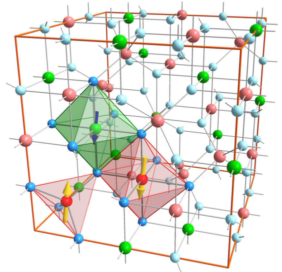
FIG. 1. (Color online) Schematic representation of the inverse spinel lattice of \text{NiFe}_2\text{O}_4 : \text{Fe}^{3+} cations (red) are distributed equally across tetra- ( T_d ) and octahedral ( O_h ) lattice sites, while \text{Ni}^{2+} cations (green) occupy O_h sites. An antiferromagnetic coupling between the T_d and O_h sites compensates the magnetic moments of the \text{Fe}^{3+} cations, which is why only the \text{Ni}^{2+} cations account for the net macroscopic magnetization of 2 \mu_B/\text{f.u.} (where f.u. denotes formula units).
