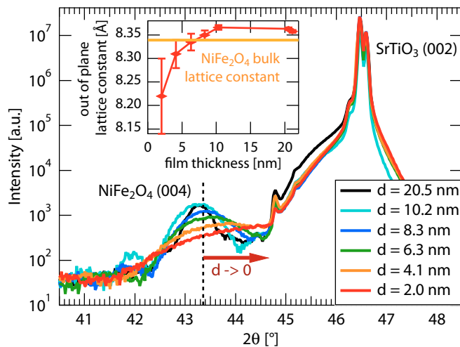
FIG. 2. (Color online) \theta - 2\theta scans of the \text{NiFe}_2\text{O}_4 (004) reflection for varying film thickness. The out-of-plane lattice constant a_{\text{oop}} decreases below the bulk value for ultrathin films (see inset).
