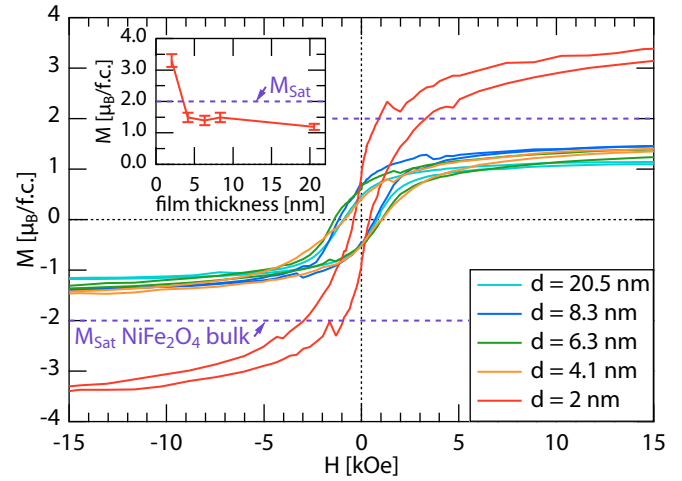
FIG. 3. (Color online) Details of the in-plane M - H hysteresis loops of \text{NiFe}_2\text{O}_4 on \text{SrTiO}_3 (001) recorded at T = 5 \text{ K} with a maximum applied field of up to 36 kOe. The inset shows the saturation magnetization M_S as a function of \text{NiFe}_2\text{O}_4 film thickness.
