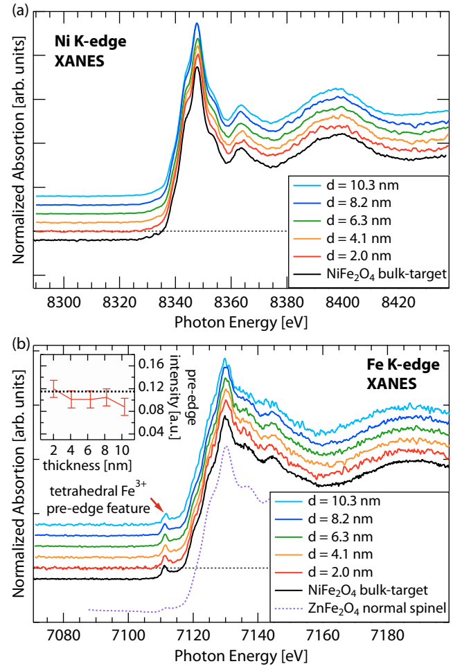
FIG. 5. (Color online) XANES spectra of (a) the Ni K edge and (b) the Fe K edge from \text{NiFe}_2\text{O}_4 films with varying film thickness. For comparison a Fe K edge spectrum of zinc ferrite, which exhibits the normal spinel structure, is plotted (reproduced from Ref. [34]). The inset in (b) shows the integrated spectral weight of the Fe K edge pre-edge feature in dependence of the film thickness, where the dotted line represents the bulk value.
