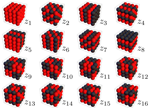
FIG. 2 (color online). The first 16 Hadamard vectors for hierarchical probing on a 4^3 lattice; red = +1, black = -1.
