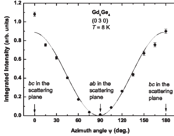
Figure 13: The integrated intensity of the (0\ 3\ 0) magnetic peak normalized by the (0\ 4\ 0) charge peak at T = 8\text{ K} . The solid curve represents the variation expected for magnetic moments along the c axis. The Figure has been taken from Ref.[32].
