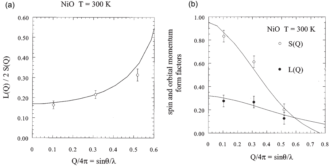
Figure 18: (a) Measured variation of L(\vec{Q})/2S(\vec{Q}) as a function of \sin\frac{\theta}{\lambda} = \frac{Q}{4\pi} . The continuous line is the K dependence estimated by Blume [Ref. [54]] adjusted to fit through the data with a contraction of the wave function by 17%. L(\vec{Q})/2S(\vec{Q}) extrapolates to 0.17 at \vec{Q} = 0 . (b) Spin form factor and orbital-moment form factor in NiO. The data have been obtained by normalizing magnetic intensities to charge peaks corrected for extinction. The continuous lines are the calculated variations of S(\vec{Q}) and L(\vec{Q}) with \sin\frac{\theta}{\lambda} from Refs. [54] and [55] with an expansion of the \vec{Q} scale by 17%.
