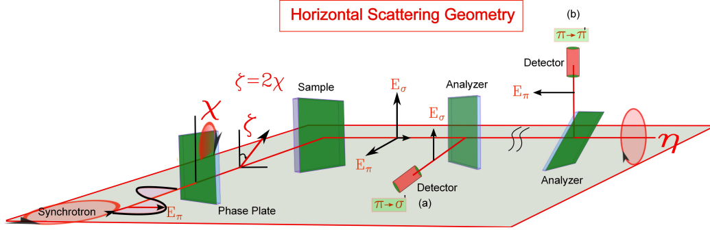
Figure 4: Experimental realization of different polarization channels for the (a) \pi \rightarrow \sigma' and (b) \pi \rightarrow \pi' scattering geometries.
