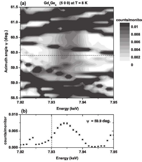
Figure 14: (a) Contour map of the intensity as a function of energy and azimuth angle \psi at the (5 0 0) position and T = 8 K. Discontinuities in the bands of multiple scattering across the energy range are artifacts of the scanning process and (b) single energy scan at the azimuth angle \psi = 59.9^\circ , which is depicted as a horizontal dashed line in (a). In (b), the vertical dashed line represents the position of the Gd L_{II} absorption edge. Figure adapted from Ref. [32].
