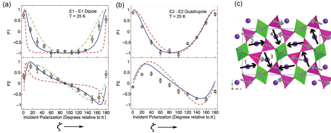
Figure 16: (a) A plot of the measured Poincaré-Stokes parameters P_1 and P_2 as a function of the incident x-ray polarization of the commensurate reflection (4+\delta, 4, 0-\tau) at the E1-E1 (dipole) energy resonance at 25 K. Simulations of the \text{Mn}^{4+} and \text{Mn}^{3+} magnetic structures as refined by Blake et al. [Ref. [41]] are shown as blue solid and red dashed lines, respectively. A simulation of the terbium magnetic structure scattering at the E1-E1 transition in this phase, as refined in Fig. (b) at the E2-E2 transition, is shown by the green dash-dotted line. (b) A plot of the measured Poincaré-Stokes parameters P_1 and P_2 as a function of incident x-ray polarization of the commensurate (4+\delta, 4, 0-\tau) reflection at the E2-E2 (quadrupole) energy resonance at 25 K. (c) Diagrammatic illustration of the refined terbium ion magnetic-moment directions (black arrows) in the CM phase. Figures taken from Ref. [42].
